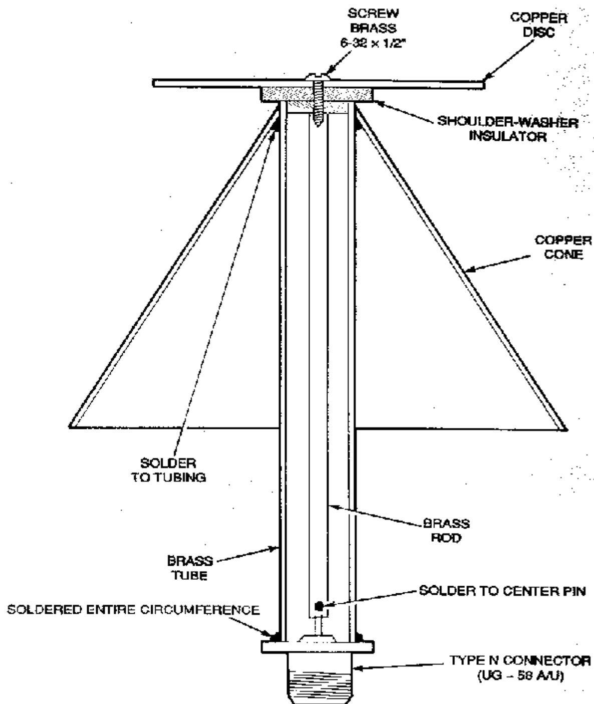
Fig 3 Discone Construction
