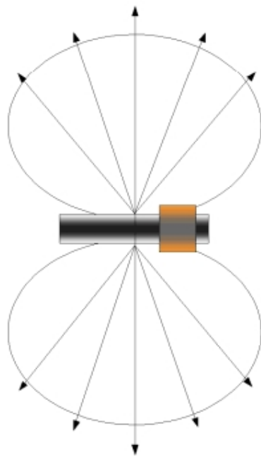
Antenna with short length and bigger diameter
