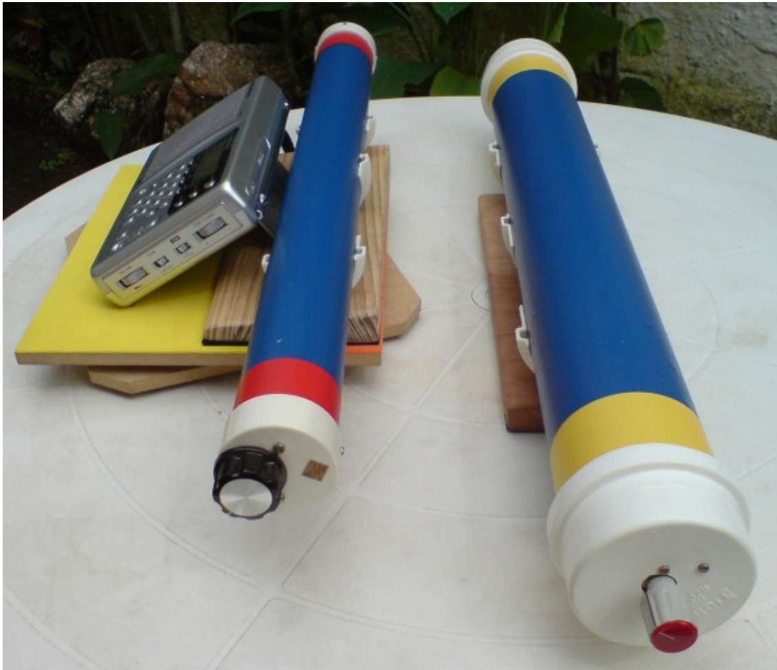
Comparing the 3 antennas, the original RGP3 and both extended loops, showed improvements only in the larger one
