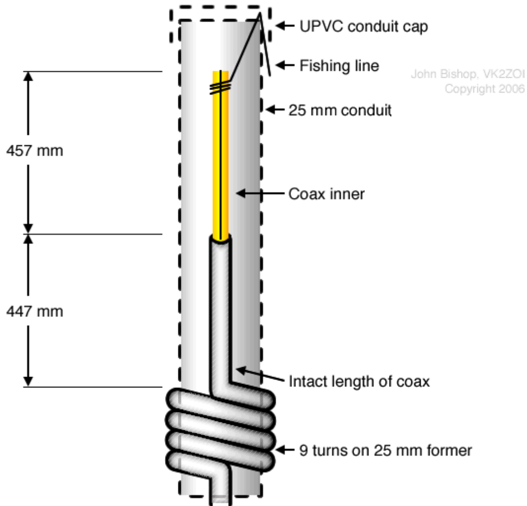
Basic arrangement of the 2m Half-Wave version
