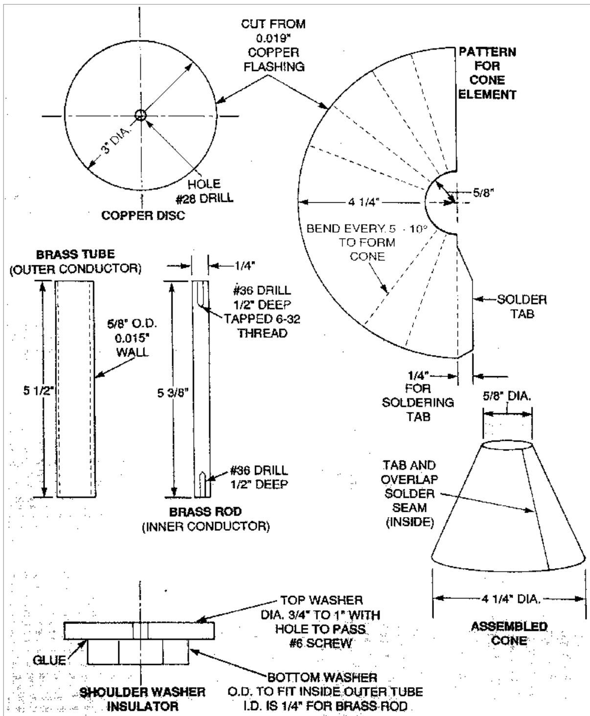
Fig 2 Discone Parts
