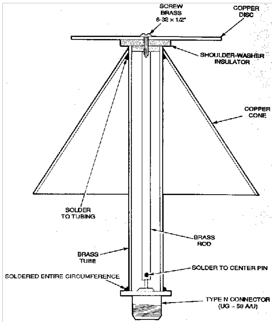
Fig 3 Discone Construction
