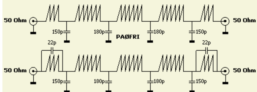
2kW low-pass filter 1.8-30MHz
