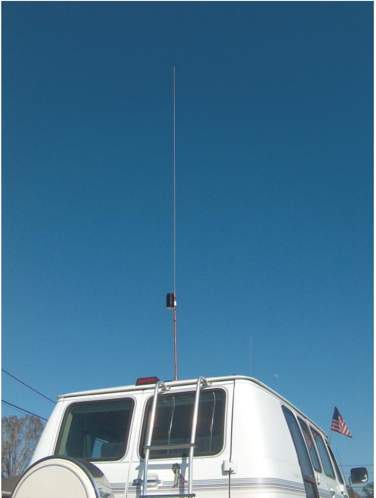
The 40 meter loading coil installed on the antenna.
