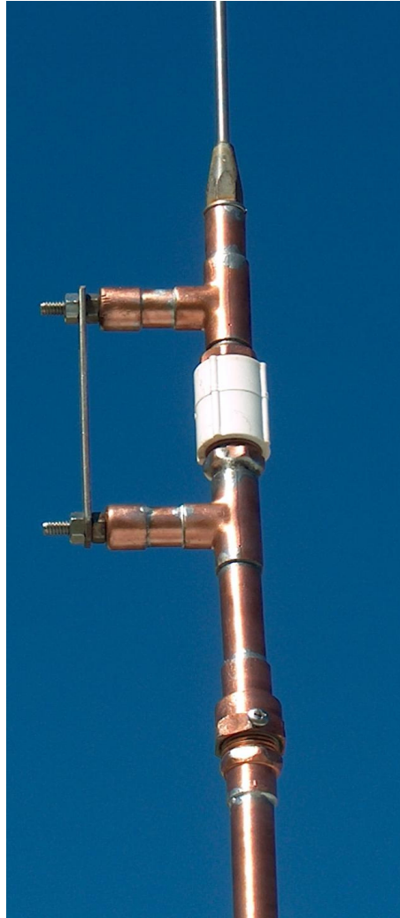
The coil support posts shown with the 10 - 12 - 15 meter shunt strap in place.
