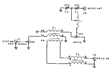
Fig. 3 Noise balancing bridge. C1, C2: 370 pF compression-type trimmer with shaft (air capacitors may be used). L1: 45 turns No. 22 enamel wire, 1-inch in diameter, turns spaced wire diameter. T1: 16 turns No. 18, trifilar wound on 3/4-inch diameter ferrite core, Q2 material (permeability of 125). J.W. Miller F-125-2 or Amidon FT-82-61. T2: Same core material, 18 turns No. 18 bifilar wound. Note: dots on drawing indicate adjacent ends of windings.
