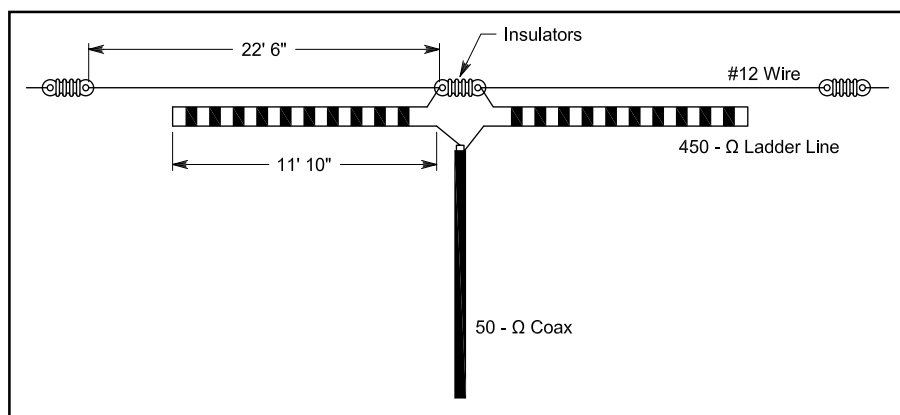
Figure 1—Layout of K4VX linear-loaded dipole. Although the #12 wire is threaded through the 450- \Omega window line to support it, this is not shown in this drawing for clarity.
