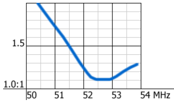
VSWR plot of the 6m Half-Wave antenna
