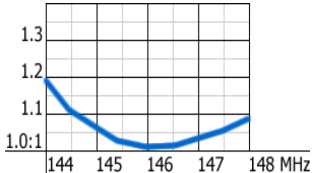
VSWR plot of the 2m Half-Wave antenna
