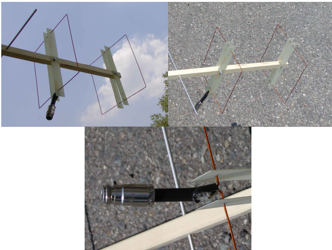
Fig. 9 IK1HGE 432MHz 8el Quagi - Prototype construction details
