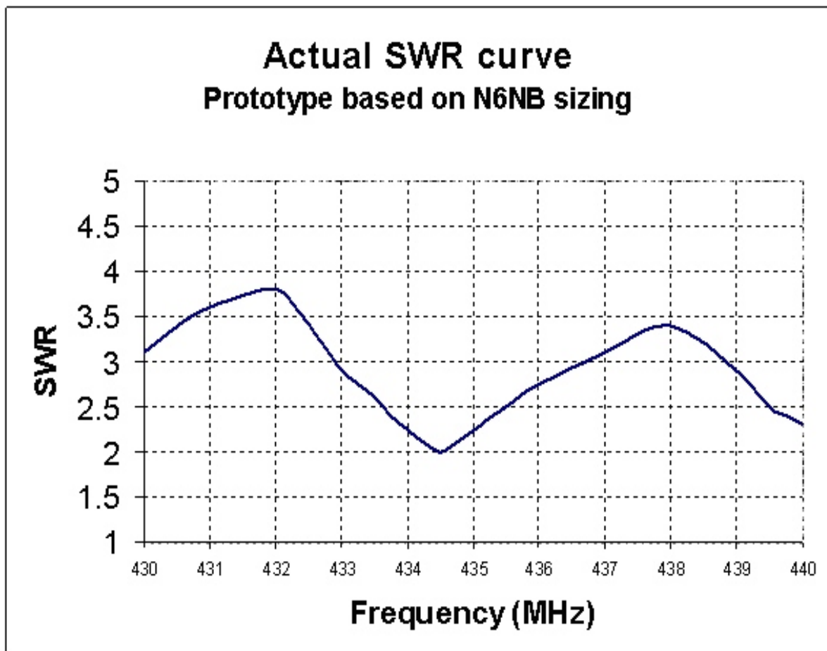
Fig. 1 Experimental SWR curve obtained with N6NB's design (materials as specified in the text above)
