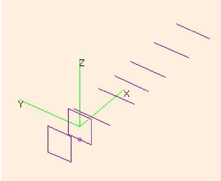
Fig. 2 Structure of the quagi antenna
