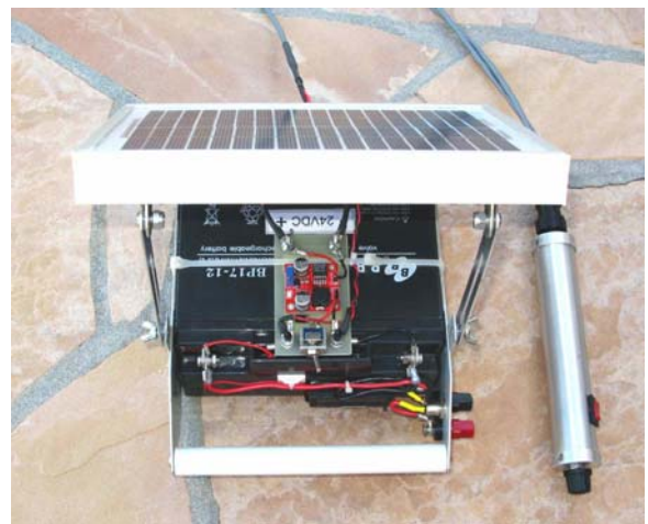
12v gel cell transceiver supply, with 12v to 24v switching supply DC-DC module, www.lightobject.com for the gearmotor drive
