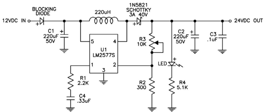
SIMPLE SWITCHER – STEP UP REGULATOR Input: 3.5V ~ 35V, Output: 4.5V ~ 35V up to 2.5A
