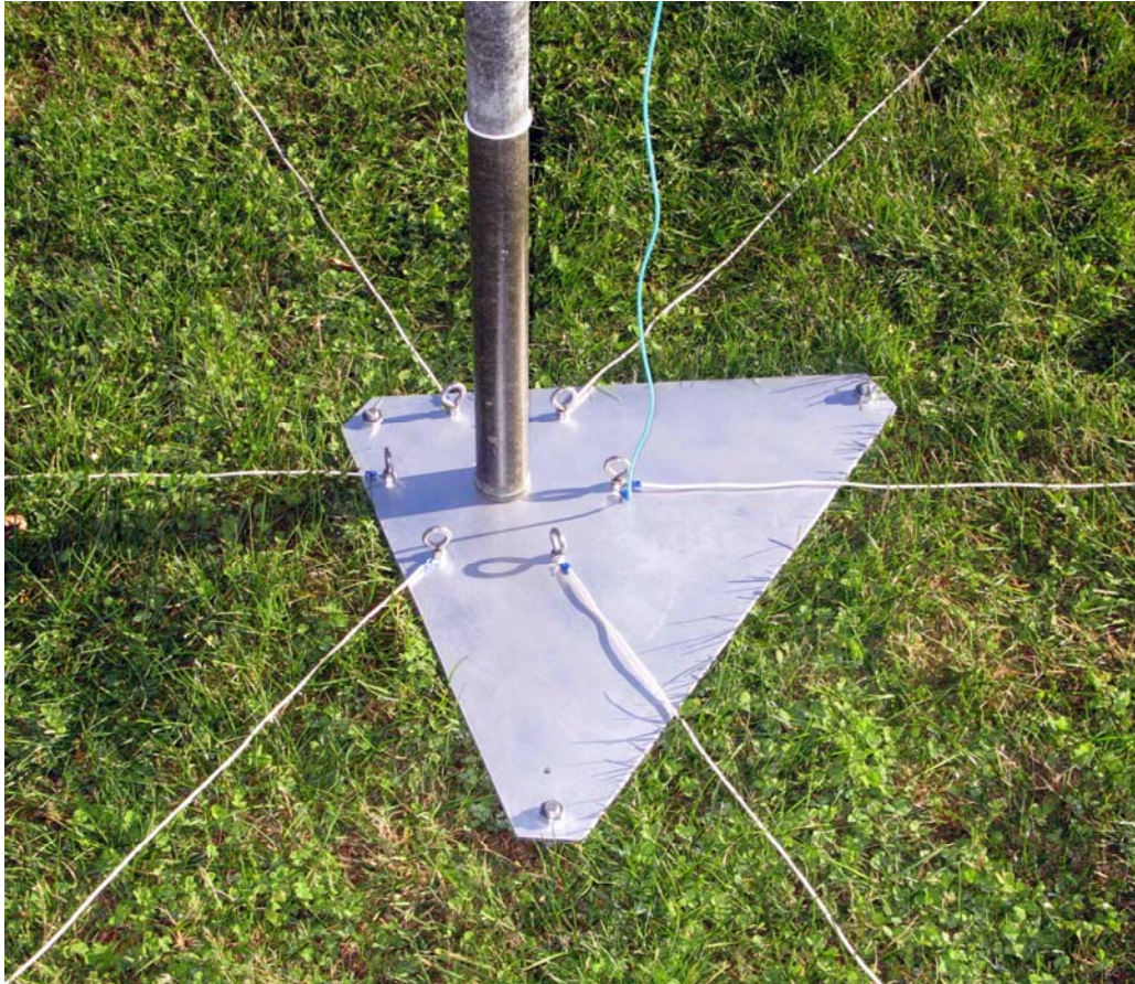
Base with thumbscrews for 6' radials, and surplus fiberglass mast section.
