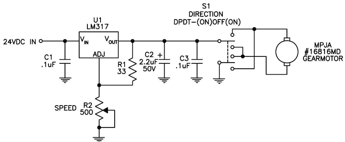
Motor controller, direction and speed
