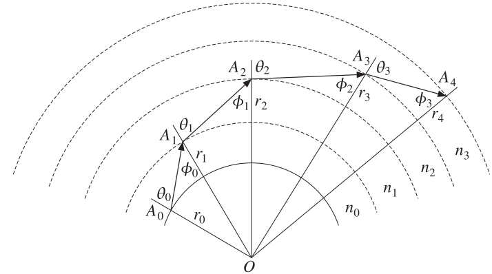
Fig. 6.11.6 Ray tracing in spherically stratified medium.
