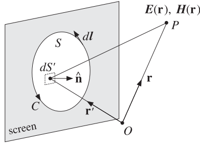
Fig. 16.12.1 Aperture surface S bounded by contour C .
