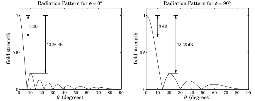
Fig. 16.8.2 Radiation patterns along the two principal planes ( a = 8\lambda, b = 4\lambda ).
