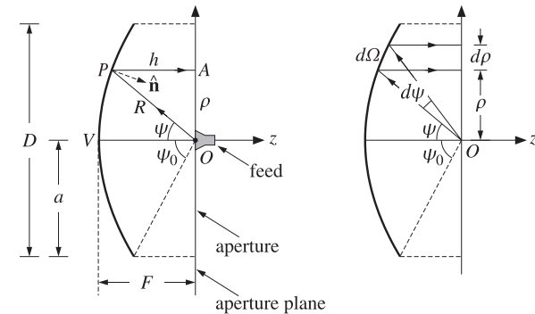
Fig. 17.7.1 Parabolic reflector antenna with feed at the focus.
