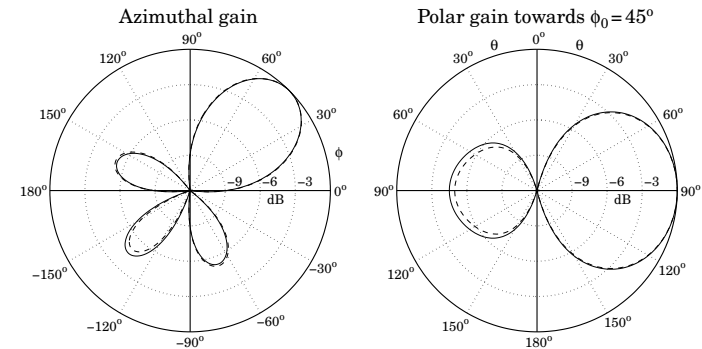
Fig. 21.4.4 H-plane and E-plane radiation patterns, \mathbf{V} = [0, 1, 1]^T .
