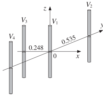
Fig. 21.4.5 Four-element parasitic array.
