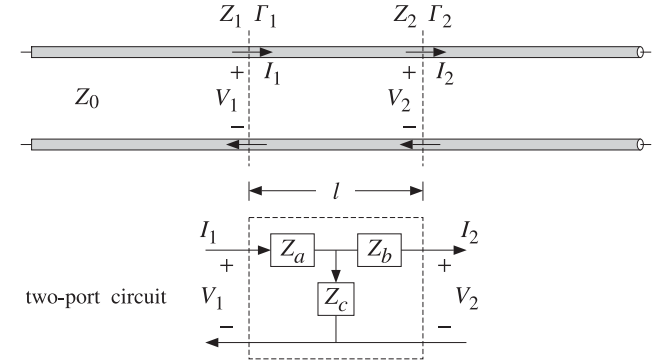
Fig. 9.8.1 Length- l segment of a transmission line and its equivalent T -section.
