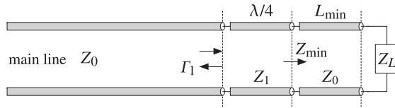
Fig. 11.5.1 Quarter-wavelength transformer for matching a complex load.
