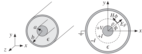
Fig. 9.4.1 Coaxial transmission line.
