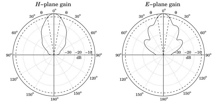
Fig. 17.3.2 H - and E -plane gains for A = 4\lambda , B = 3\lambda , and \sigma_a = 1.2593 , \sigma_b = 1.0246 .
