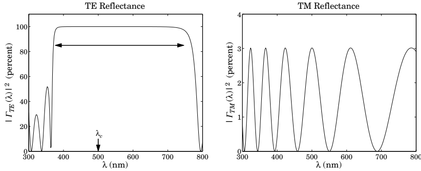
Fig. 7.6.2 Polarizer with n_H = 2.3 and n_L = 1.25 .
