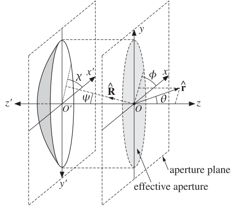
Fig. 17.7.2 Parabolic antenna and its projected effective aperture.
