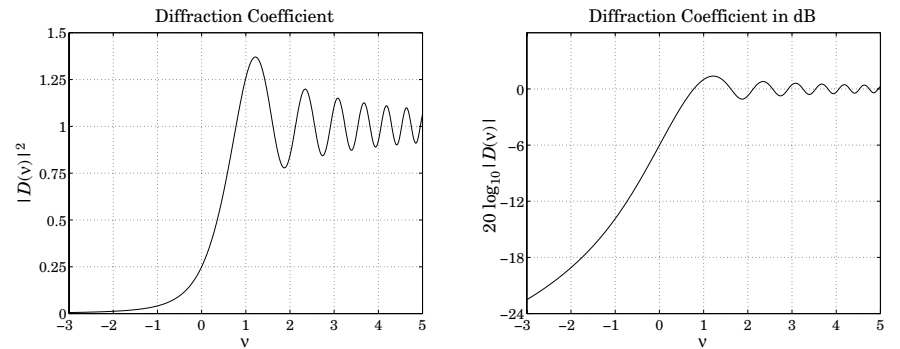
Fig. 16.14.2 Diffraction coefficient in absolute and dB units.
