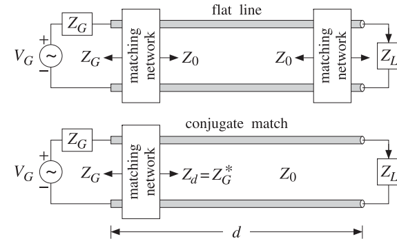
Fig. 11.1.1 Reflectionless and conjugate matching of a transmission line.
