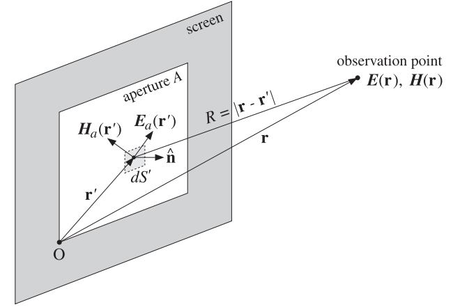
Fig. 16.1.1 Radiated fields from an aperture.
