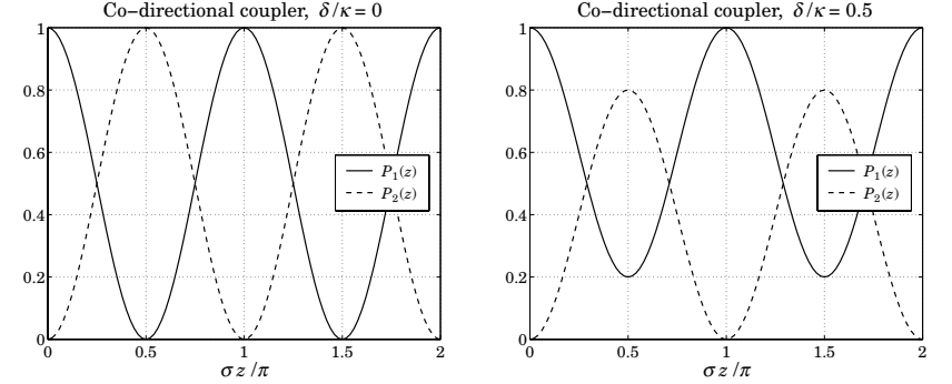
Fig. 10.4.2 Power exchange in co-directional couplers.
