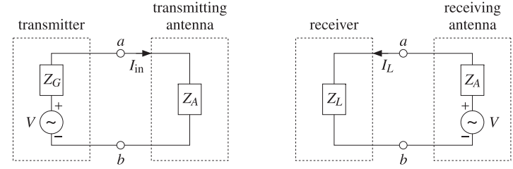
Fig. 14.4.1 Circuit equivalents of transmitting and receiving antennas.
