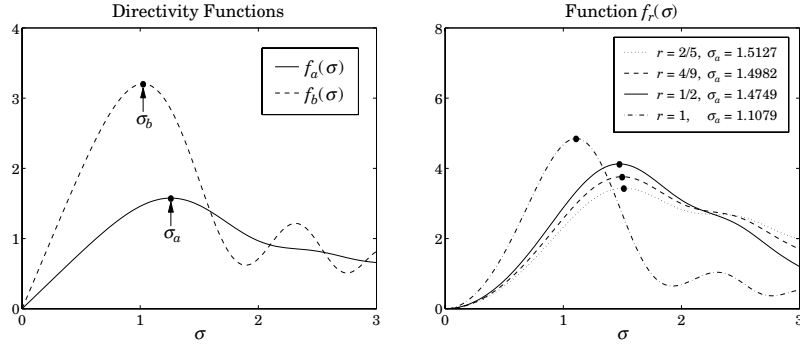
Fig. 17.4.1 Directivity functions.
