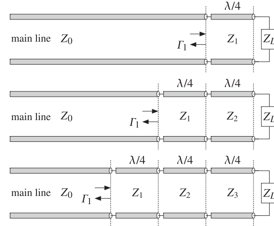
Fig. 11.3.1 One, two, and three-section quarter-wavelength transformers.
