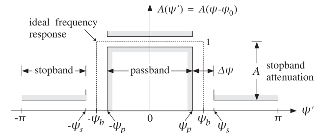
Fig. 19.4.1 Specifications of equivalent lowpass response.
