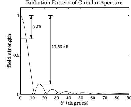
Fig. 16.9.2 Radiation pattern of circular aperture ( a = 3\lambda ).
