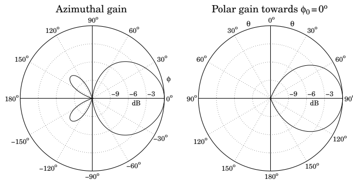
Fig. 21.4.6 H-plane and E-plane radiation patterns, \mathbf{V} = [1, 0, 0, 0]^T .
