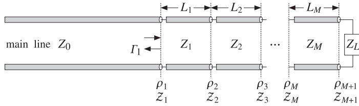
Fig. 11.2.1 Multi-section transmission line.
