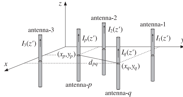
Fig. 21.4.1 Two-dimensional array of parallel dipoles.
