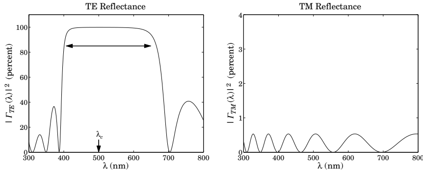
Fig. 7.6.3 Polarizer with n_H = 2.04 and n_L = 1.385 .
