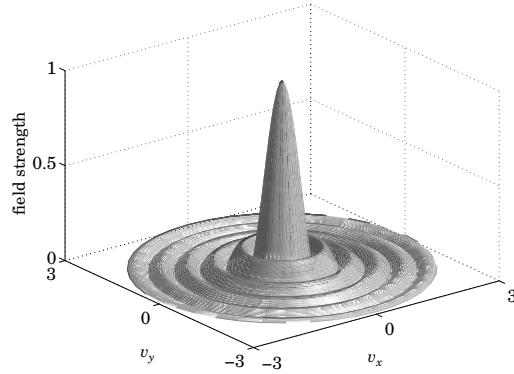
Fig. 16.9.1 Radiation pattern of circular aperture ( a = 3\lambda ).
