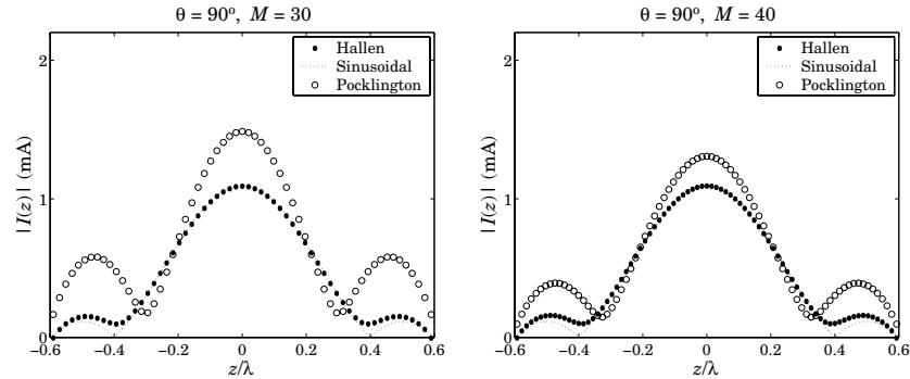
Fig. 20.10.3 Hallén and Pocklington solutions for broadside incident field.
