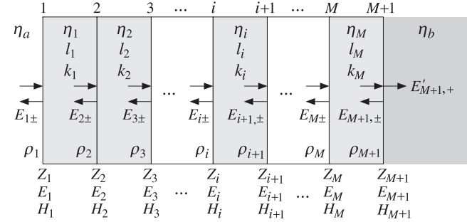
Fig. 5.1.1 Multilayer dielectric slab structure.
