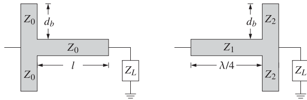
Fig. 11.9.2 Balanced microstrip single-stub and quarter-wavelength transformers.
