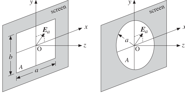
Fig. 16.7.1 Uniform rectangular and circular apertures.
