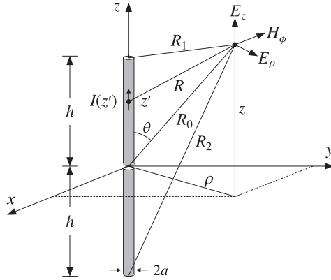
Fig. 21.1.1 Fields of a thin wire antenna.
