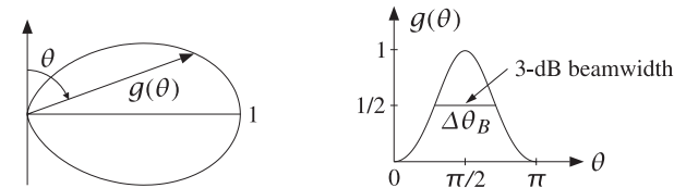
Fig. 14.2.2 Polar and regular plots of normalized gain versus angle.
