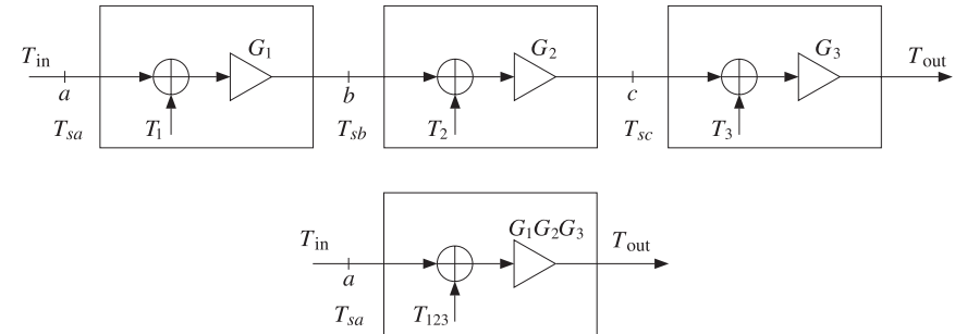
Fig. 14.8.3 Equivalent noise temperatures of three cascaded devices.
