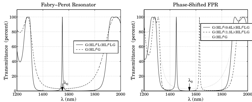
Fig. 5.5.1 Narrowband FPR transmission filters.
