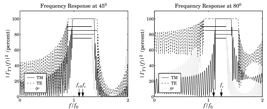
Fig. 7.5.7 Unequal length layers L_H = 0.30 , L_L = 0.15 .
