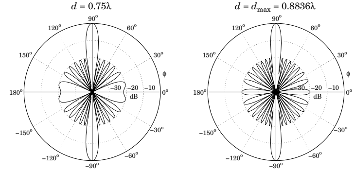
Fig. 19.8.3 Chebyshev arrays with N = 9 , R = 20 dB, d = 3\lambda/4 and d = 0.8836\lambda .
