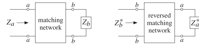
Fig. 11.13.1 Forward and reversed matching networks.
