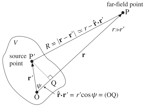
Fig. 13.7.1 Far-field approximation.
