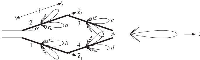
Fig. 15.7.5 Traveling-wave rhombic antenna.
