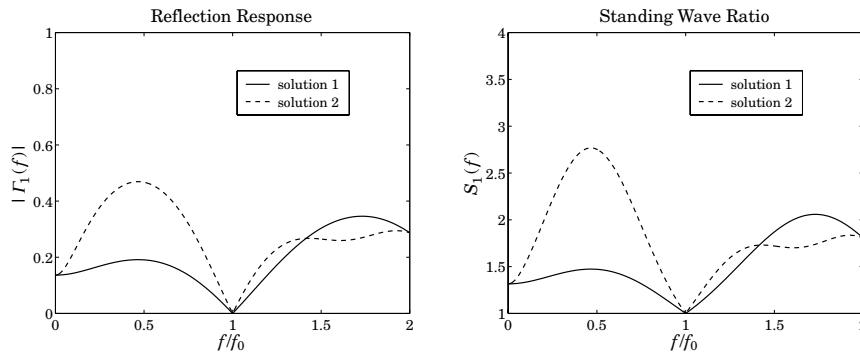
Fig. 11.7.2 Reflection response of two-section series transformer.
