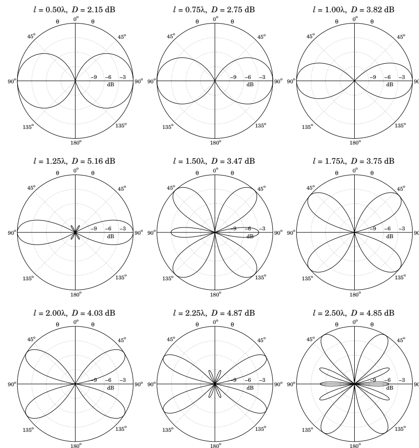
Fig. 15.4.2 Standing-wave dipole antenna patterns and directivities.
