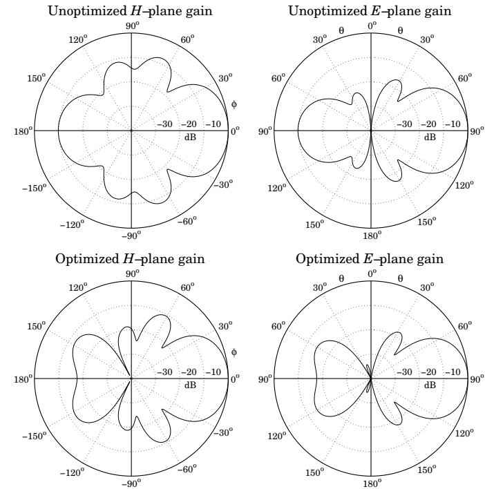
Fig. 21.5.5 Gains of six-element Yagi-Uda array.
