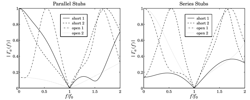
Fig. 11.8.3 Reflection response of single stub matching solutions.
