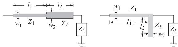
Fig. 11.6.2 Microstrip matching circuits.
