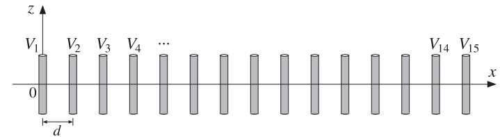
Fig. 21.4.7 Fifteen-element Dolph-Chebyshev array.
