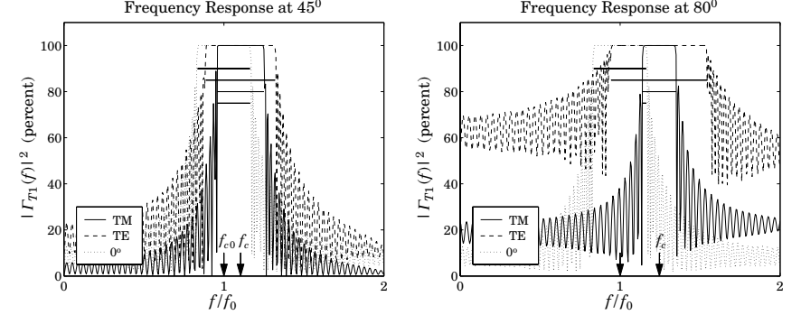
Fig. 7.5.3 TM and TE frequency responses for n_H = 2.32 , n_L = 1.38 .
