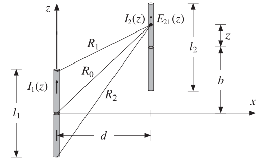
Fig. 21.2.1 Parallel linear dipoles.
