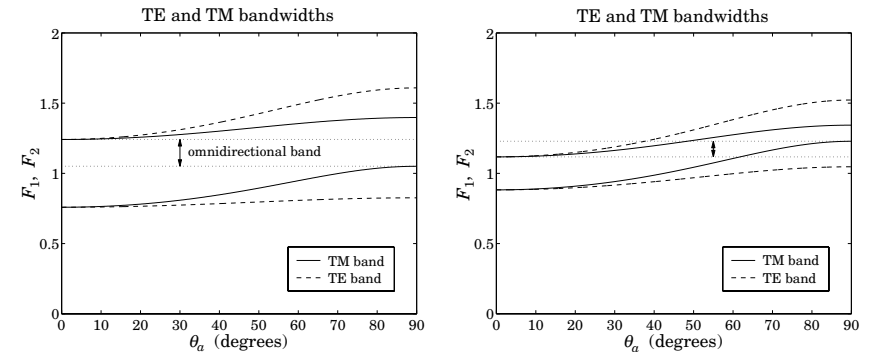
Fig. 7.5.6 TM/TE bandgaps versus angle for n_H = 3 , n_L = 1.38 and n_H = 2 , n_L = 1.38 .
