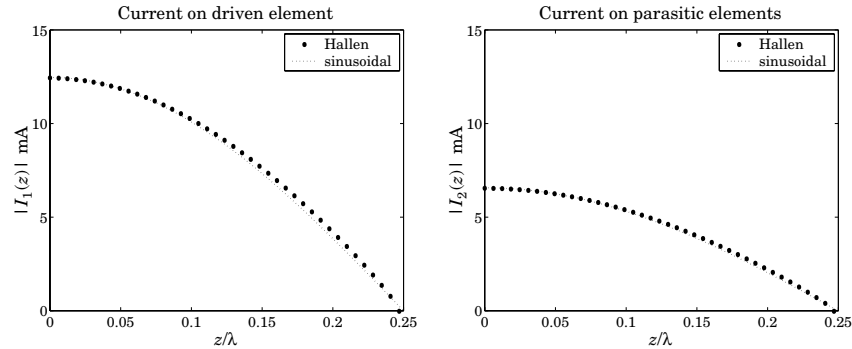
Fig. 21.6.1 Currents on driven and parasitic antennas.
