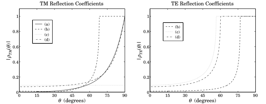
Fig. 7.8.1 TM and TE birefringent Fresnel reflection coefficients versus incident angle.
