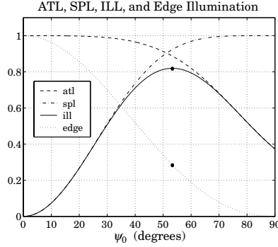
Fig. 17.8.1 Tradeoff between ATL and SPL.
