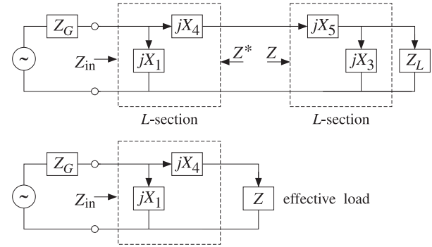
Fig. 11.12.2 Equivalent L -section networks.
