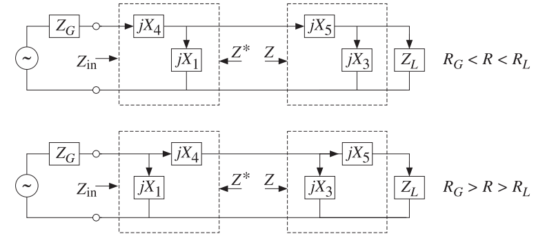
Fig. 11.12.4 Double L -section networks.
