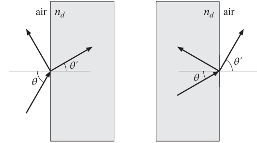
Fig. 6.4.1 Air-dielectric interfaces.
