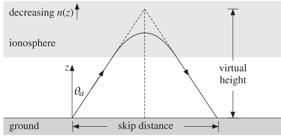
Fig. 6.11.2 Ionospheric refraction.
