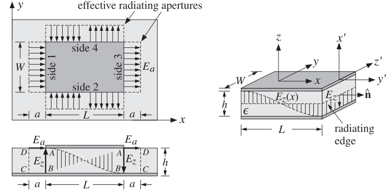
Fig. 17.6.2 Aperture models for microstrip antenna.
