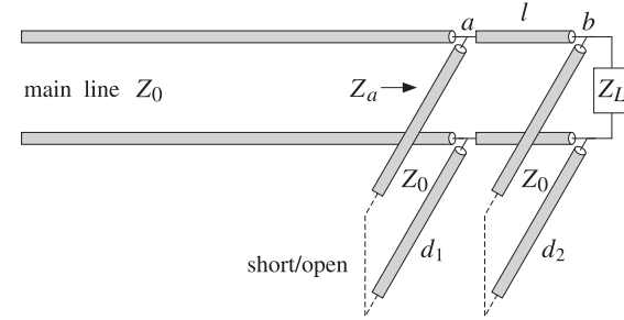
Fig. 11.10.1 Double stub tuner.
