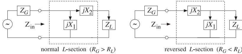
Fig. 11.11.1 L -section reactive conjugate matching network.
