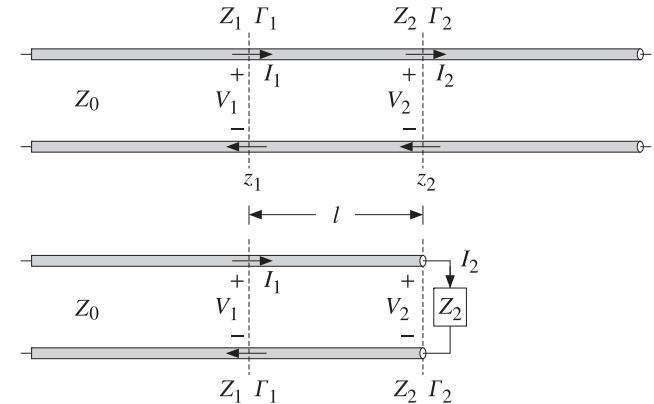
Fig. 9.7.1 Length segment on infinite line and equivalent terminated line.
