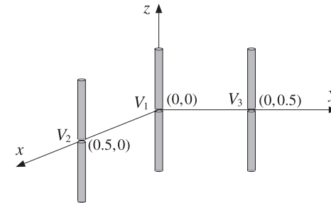
Fig. 21.4.2 Three-element array.
