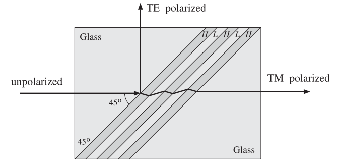
Fig. 7.6.1 Polarizing beam splitter.
