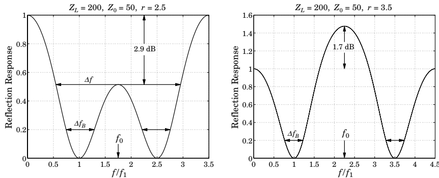
Fig. 11.4.3 Dual-band transformers at frequencies \{f_1, 2.5f_1\} and \{f_1, 3.5f_1\} .
