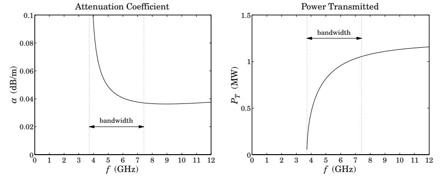
Fig. 8.8.2 Attenuation constant and transmitted power in a WR-159 waveguide.
