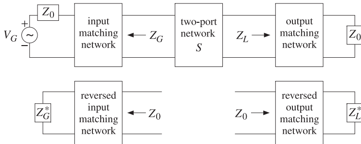
Fig. 11.13.3 Designing input and output matching networks for a two-port.
