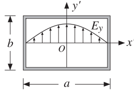
Fig. 17.1.1 Electric field over a waveguide aperture.
