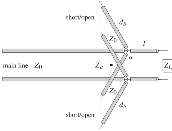
Fig. 11.9.1 Balanced stubs.
