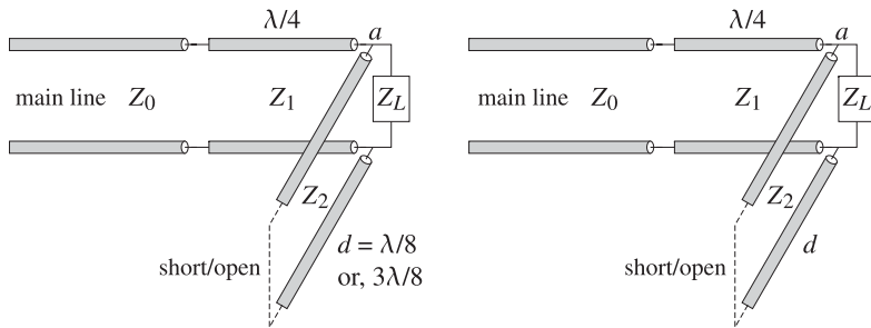
Fig. 11.6.1 Matching with a quarter-wavelength section and a shunt stub.
