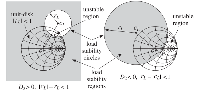
Fig. 12.5.2 Load stability regions in potentially unstable case.
