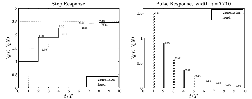
Fig. 9.15.3 Transient step and pulse responses of a terminated line.
