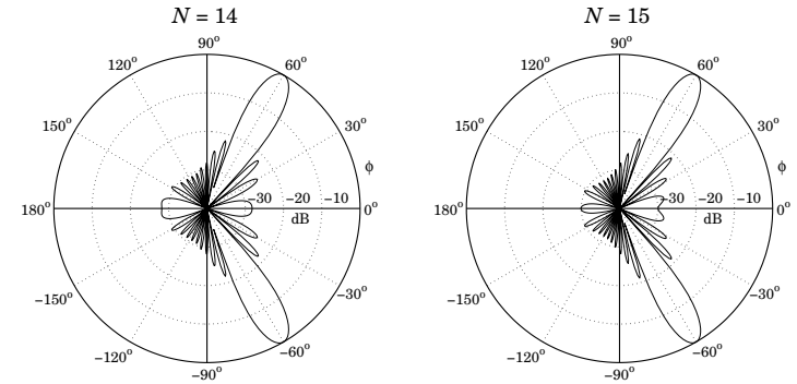
Fig. 19.9.1 Taylor-Kaiser arrays with N = 14 and N = 15 , and d = \lambda/2 .
