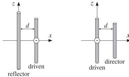
Fig. 21.5.2 The simplest Yagi-Uda arrays.
