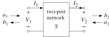
Fig. 12.1.1 Two-port network.
