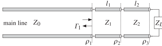
Fig. 11.4.1 Two-section dual-band Chebyshev transformer.
