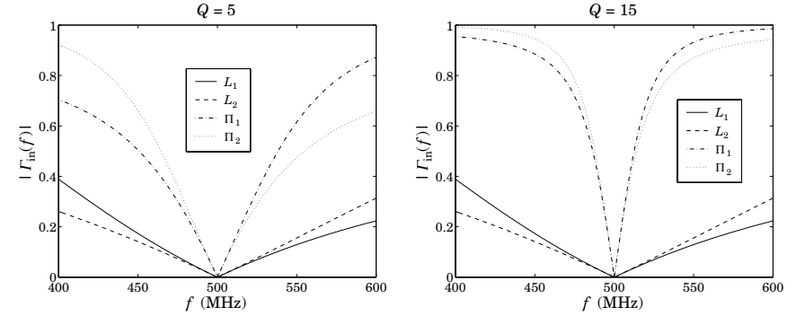
Fig. 11.12.3 Comparison of L -section and \Pi -section matching.
