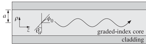
Fig. 6.11.9 Graded-index optical fiber.
