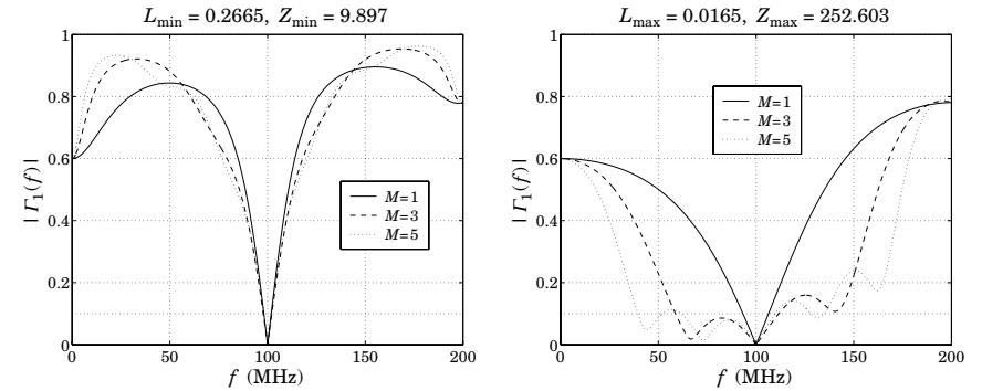
Fig. 11.5.2 Matching a complex impedance.
