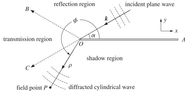
Fig. 16.15.1 Plane wave incident on conducting half-plane.
