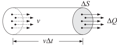
Fig. 1.5.1 Flux of a quantity.
