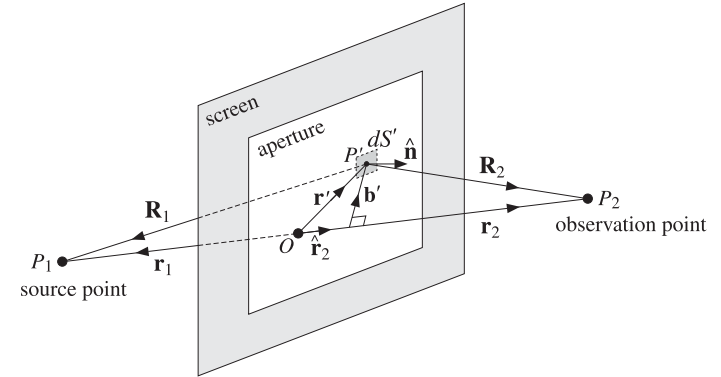
Fig. 16.13.1 Fresnel diffraction through rectangular aperture.
