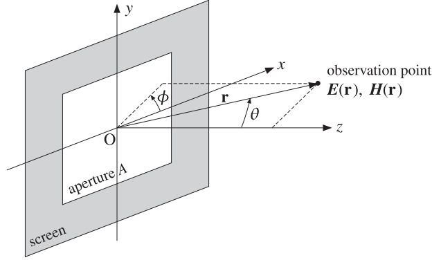
Fig. 16.4.1 Radiation fields from an aperture.
