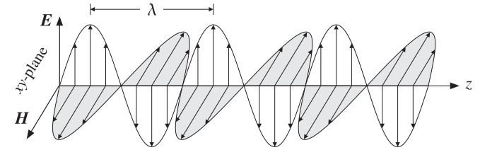
Fig. 2.2.1 Forward uniform plane wave.
