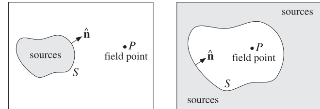
Fig. 16.10.3 Current sources are outside the field region.
