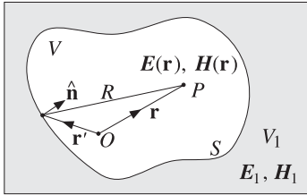
Fig. 16.10.2 Fields inside a closed surface S .
