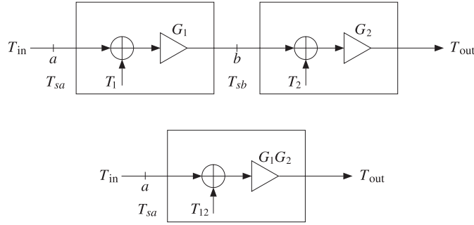
Fig. 14.8.2 Equivalent noise model of two cascaded devices.
