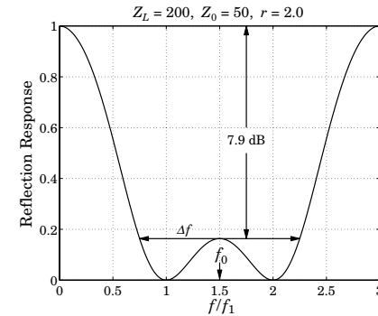
Fig. 11.4.2 Reflection response |\Gamma_1(f)|^2 normalized to unity gain at dc.
