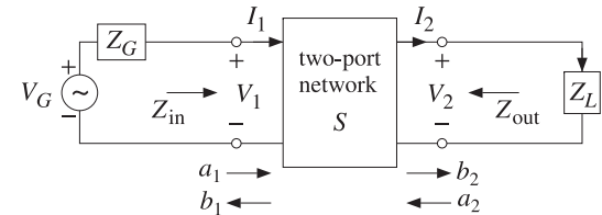
Fig. 12.1.4 Two-port network connected to generator and load.
