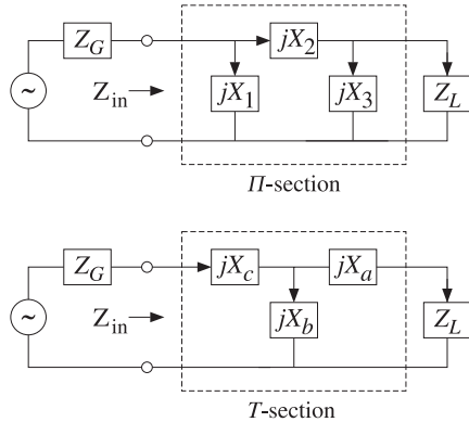
Fig. 11.12.1 \Pi - and T -section matching networks.
