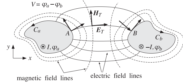
Fig. 9.1.1 Two-conductor transmission line.
