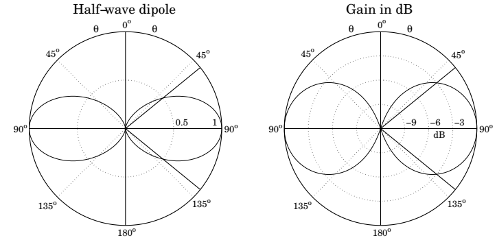
Fig. 15.4.1 Gain of half-wave dipole in absolute and dB units.
