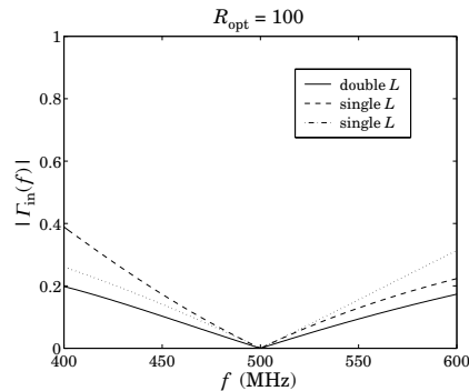
Fig. 11.12.5 Comparison of single and double L -section networks.
