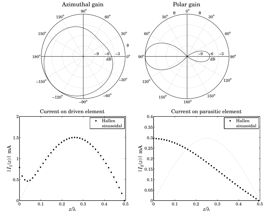
Fig. 21.6.2 Gains and currents of full-wavelength parasitic array.
