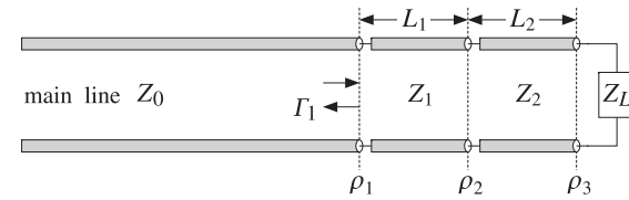
Fig. 11.7.1 Two-section series impedance transformer.
