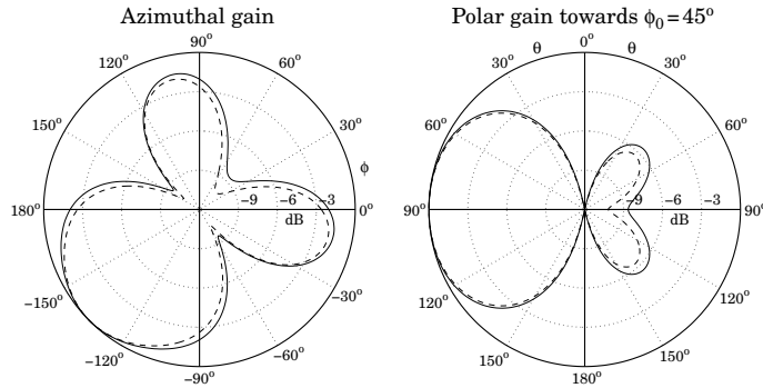
Fig. 21.4.3 H-plane and E-plane radiation patterns, \mathbf{V} = [1, 0, 0]^T .
