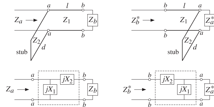
Fig. 11.13.2 Examples of reversed matching networks.
