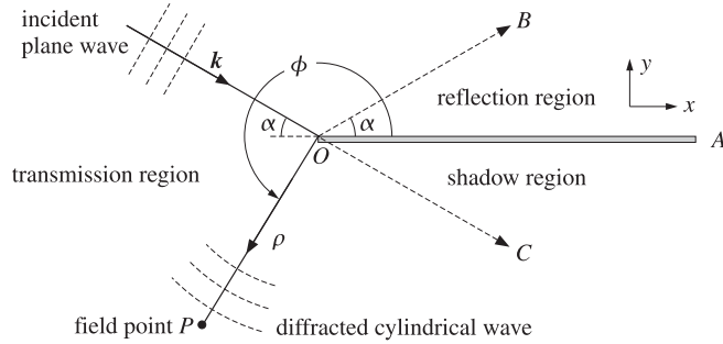
Fig. 16.15.2 Plane wave incident on conducting half-plane.
