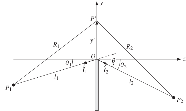
Fig. 16.14.4 Fresnel diffraction by straight edge.
