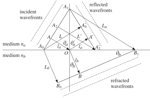
Fig. 6.10.1 Snell's laws of reflection and refraction.
