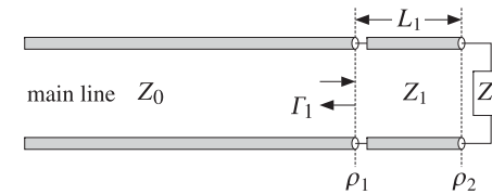
Fig. 11.7.3 One-section series impedance transformer.
