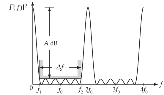
Fig. 5.8.1 Reflectance specifications for Chebyshev design.
