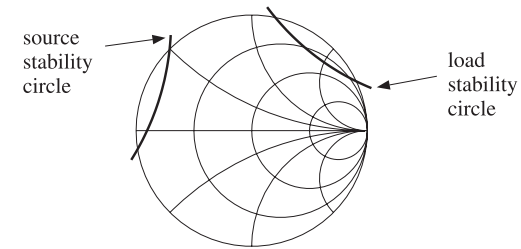
Fig. 12.5.3 Load and source stability circles at 1 GHz.
