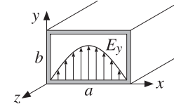
Fig. 8.4.2 Electric field inside a rectangular waveguide.
