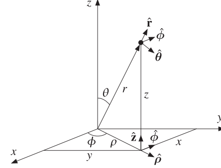
Fig. 13.8.1 Cartesian, cylindrical, and spherical coordinates.
