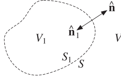
Fig. 16.11.1 Current sources may exist in both V and V_1 .
