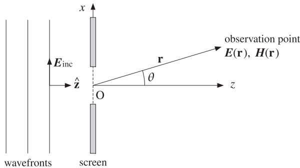
Fig. 16.5.1 Uniform plane wave incident on an aperture.
