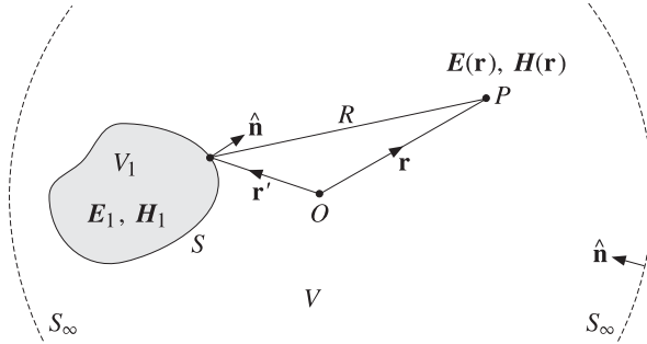
Fig. 16.10.1 Fields outside a closed surface S .
