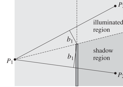
Fig. 16.14.1 Illuminated and shadow regions in straight-edge diffraction.
