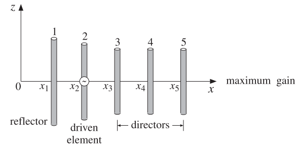
Fig. 21.5.1 Five-element Yagi-Uda array.
