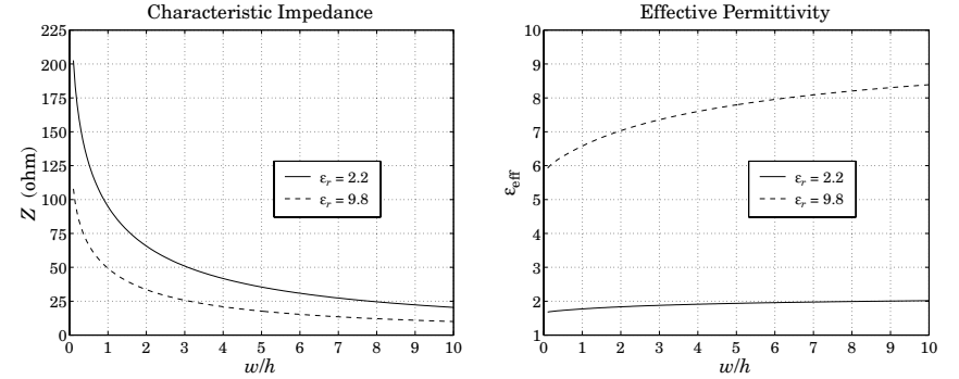
Fig. 9.3.2 Characteristic impedance and effective permittivity of microstrip line.
