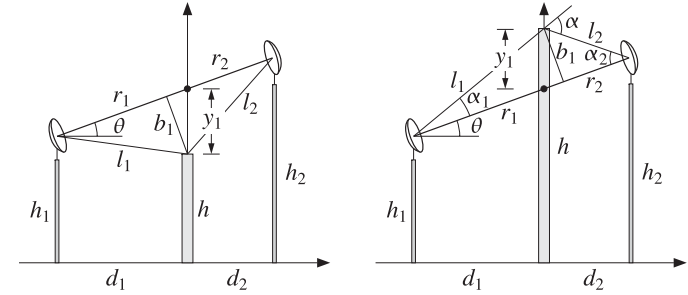
Fig. 16.14.3 Communicating antennas over an obstacle.
