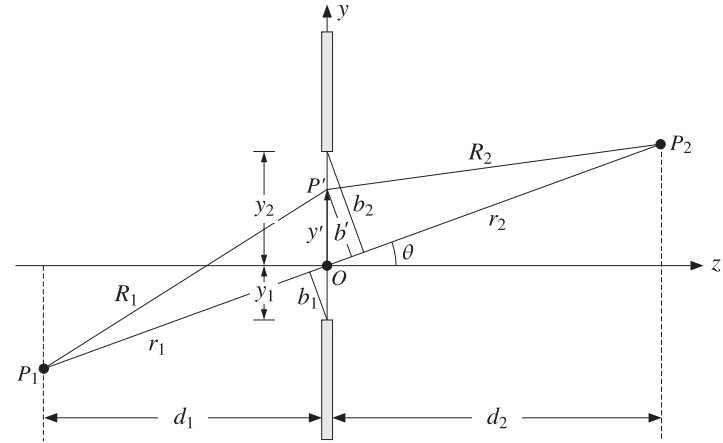
Fig. 16.13.2 Fresnel diffraction by rectangular aperture.
