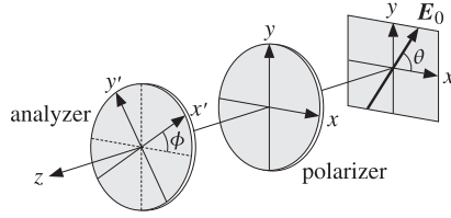
Fig. 2.12.1 Polarizer-analyzer filter combination.
