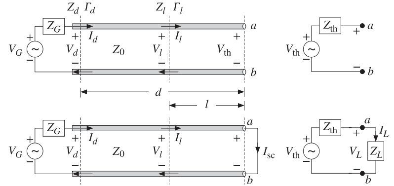
Fig. 9.11.1 Open- and short-circuited line and Thévenin-equivalent circuit.
