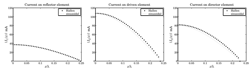
Fig. 21.6.3 Currents on the Yagi antennas.
