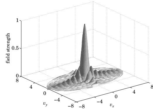
Fig. 16.8.1 Radiation pattern of rectangular aperture ( a = 8\lambda, b = 4\lambda ).
