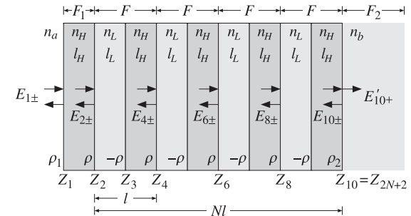
Fig. 5.3.1 Nine-layer dielectric mirror.
