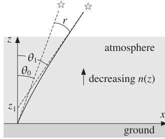
Fig. 6.11.5 Atmospheric refraction.
