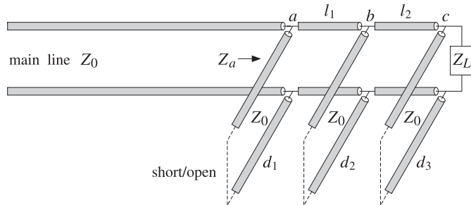
Fig. 11.10.2 Triple stub tuner.
