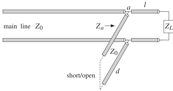
Fig. 11.8.1 Parallel connection of single stub tuner.
