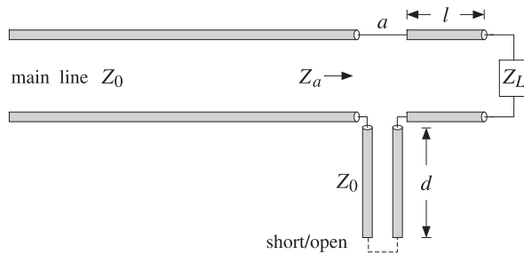
Fig. 11.8.2 Series connection of single stub tuner.
