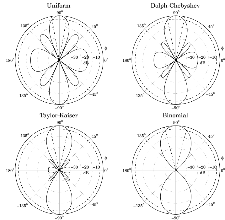
Fig. 19.6.1 Narrow beam design examples.
