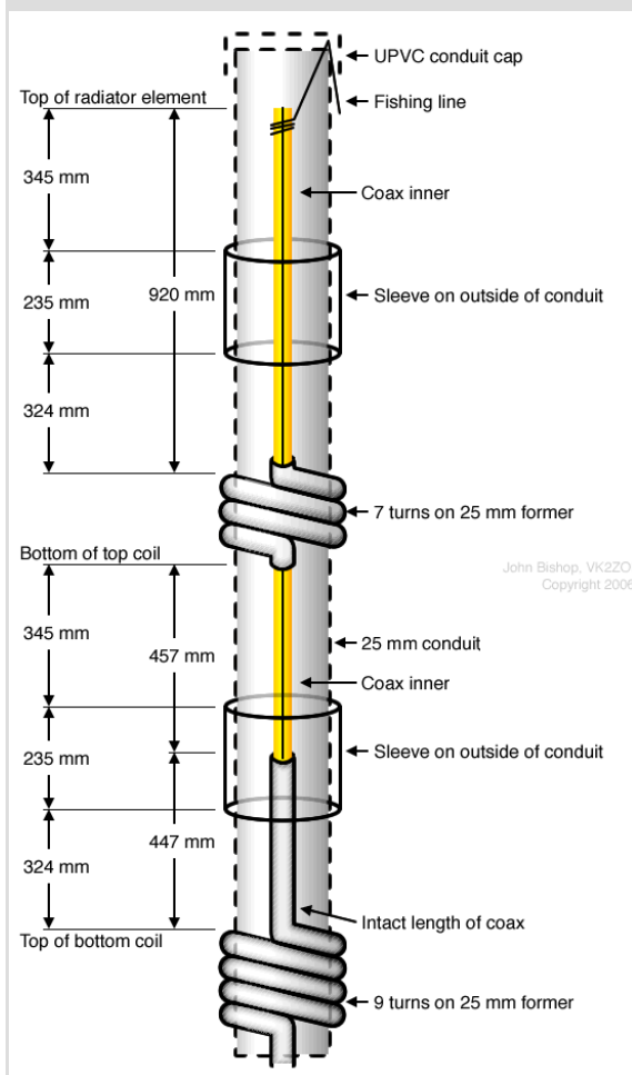
Experimental Dual Band High Gain Flower Pot dimensions
