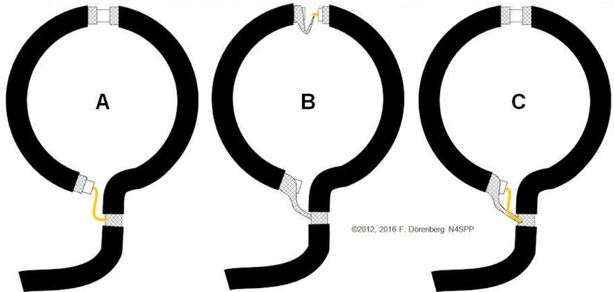
Fig. 21A: Variations of shielded coupling loops
