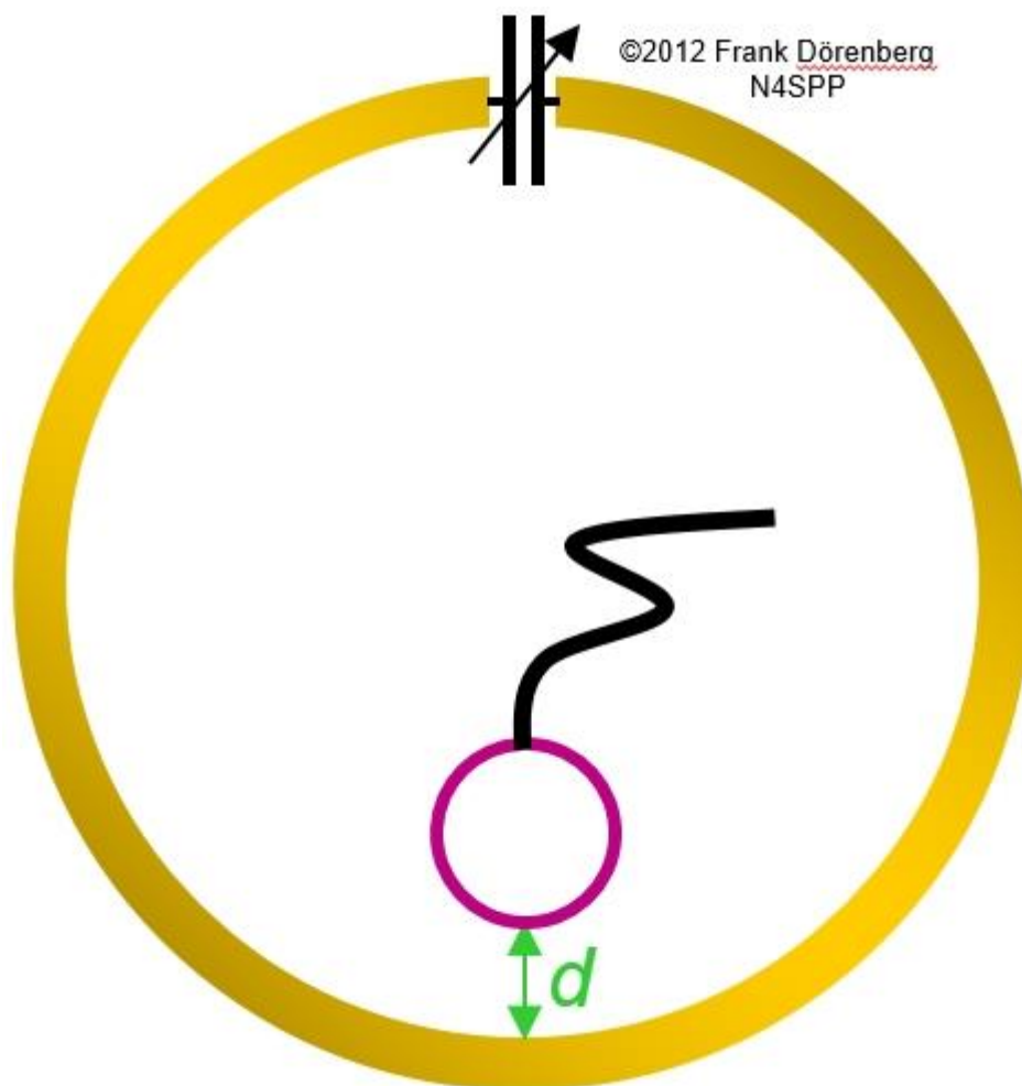
Fig. 22: The experiment of Jochen Huebl (DG1SFJ)
