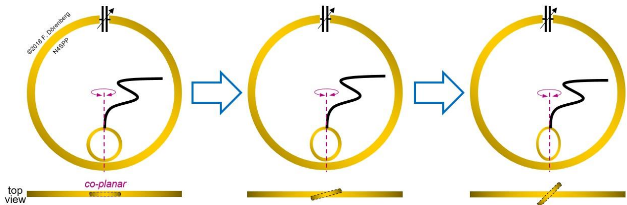
Fig. 24: turning the coupling loop about its vertical axis to change the coupling with the main loop
