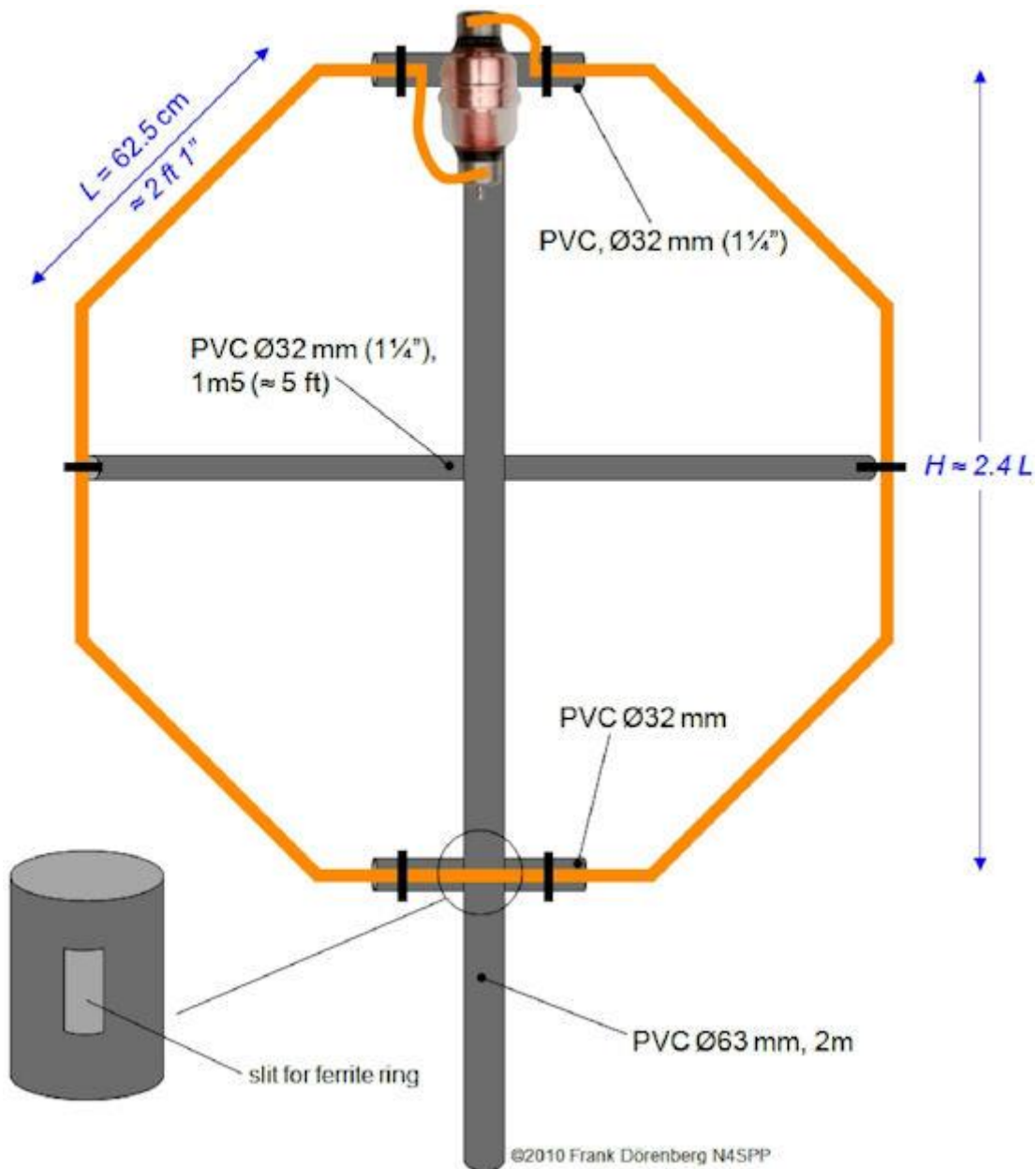
Fig. 40: The construction concept of my first STL antenna - 1.5 m (5 ft) high & wide
