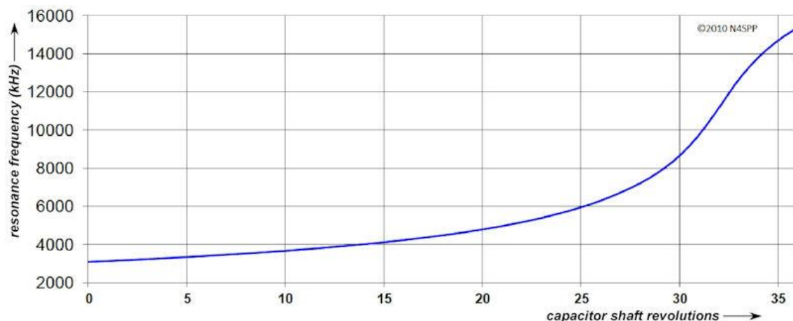
Fig. 66: Coupling transformer: FT-140-43 ferrite core - same curve for 8 & 14 secondary turns
