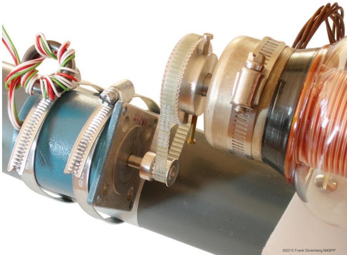
Fig. 100: The pulleys and belt installed on the motor and capacitor (note the 5-turn ferrite toroid "choke" on the motor wiring)
