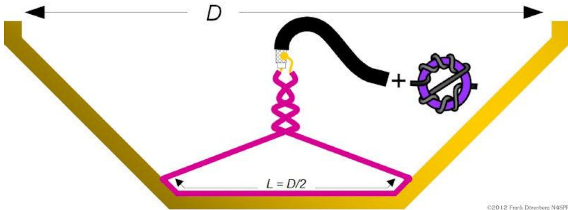
Fig. 19B: "Coat hanger" coupling loop
