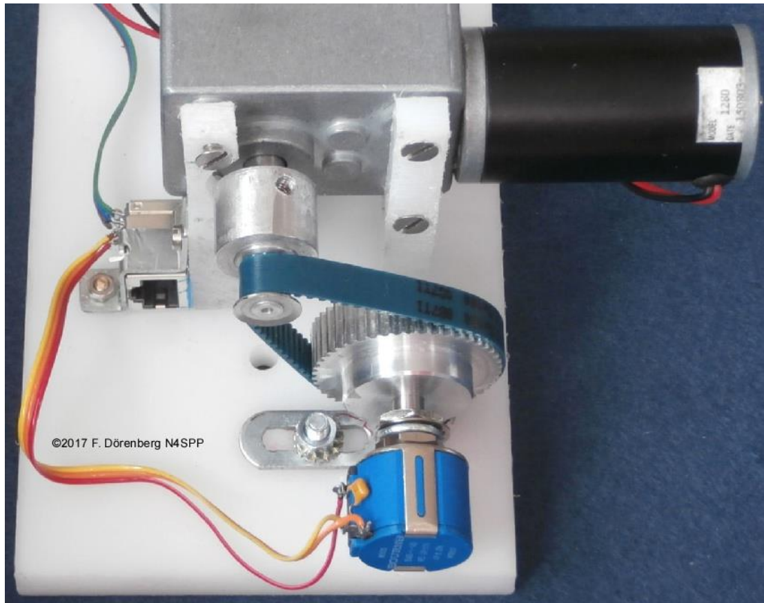
Fig. 120: The RJ45 connector and second output shaft of the motor's gear box with 4:1 belt drive to the 10-turn potmeter
