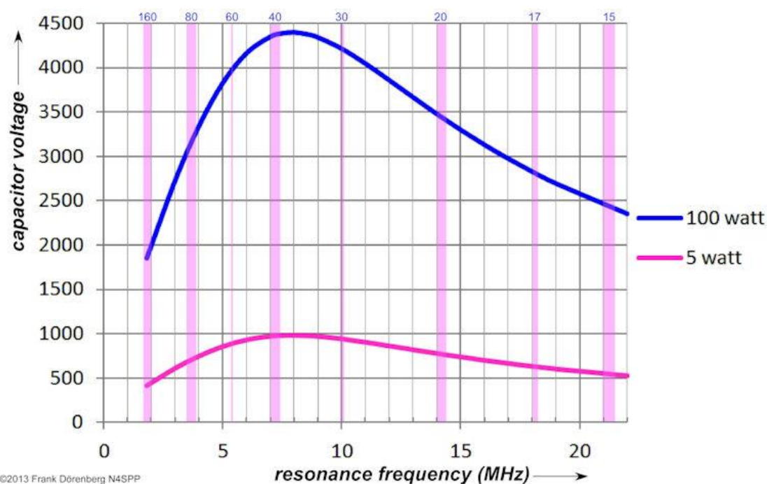
Fig. 8: Capacitor voltage as a function of frequency (1.6 mtr Ø loop made of 16 mm OD copper tubing) (calculated with ref. 2B; assumed 5 milliohm loss resistance - note: read ref. 2F for caveats about calculators!)
