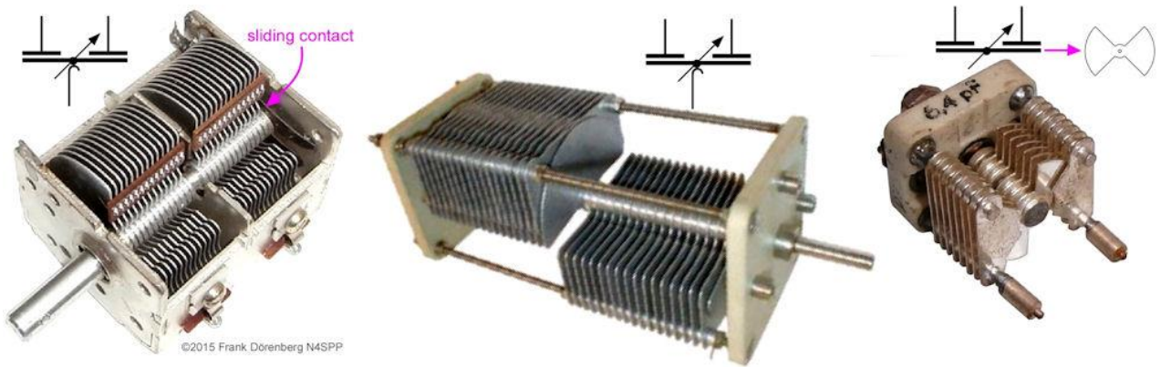
Fig. 11B: Broadcast receiver capacitor, split-stator capacitor, and butterfly trimmer
