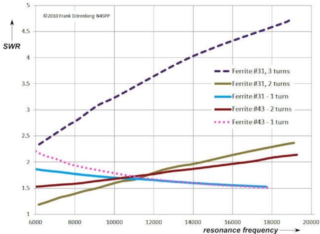
Fig. 29: SWR plot of my third STL antenna (40-10) , with ferrite cores FT-140-43 and FT-240-31
