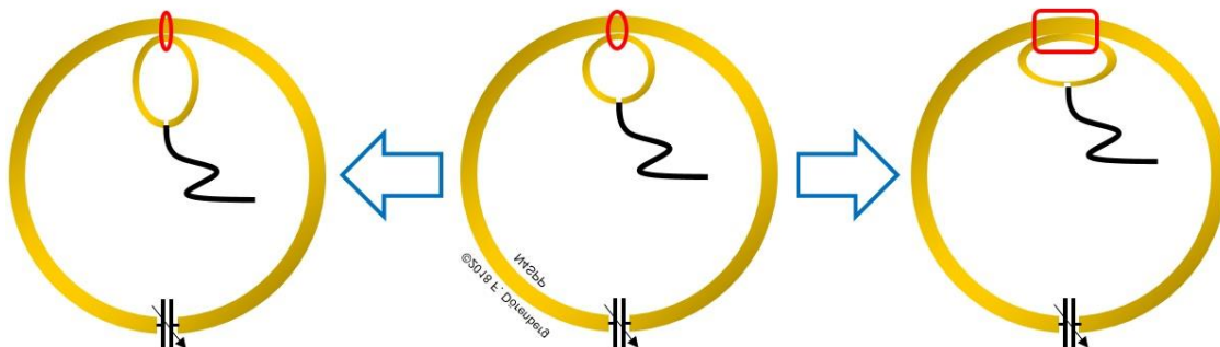
Fig. 19A: Stretching or compressing a round coupling loop to change the coupling with the main loop
