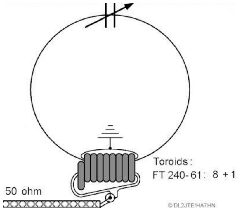
Fig. 30: Transformer-coupling per Lásló (DL2JT/HA7HN) (source: ref. 6C/D)
