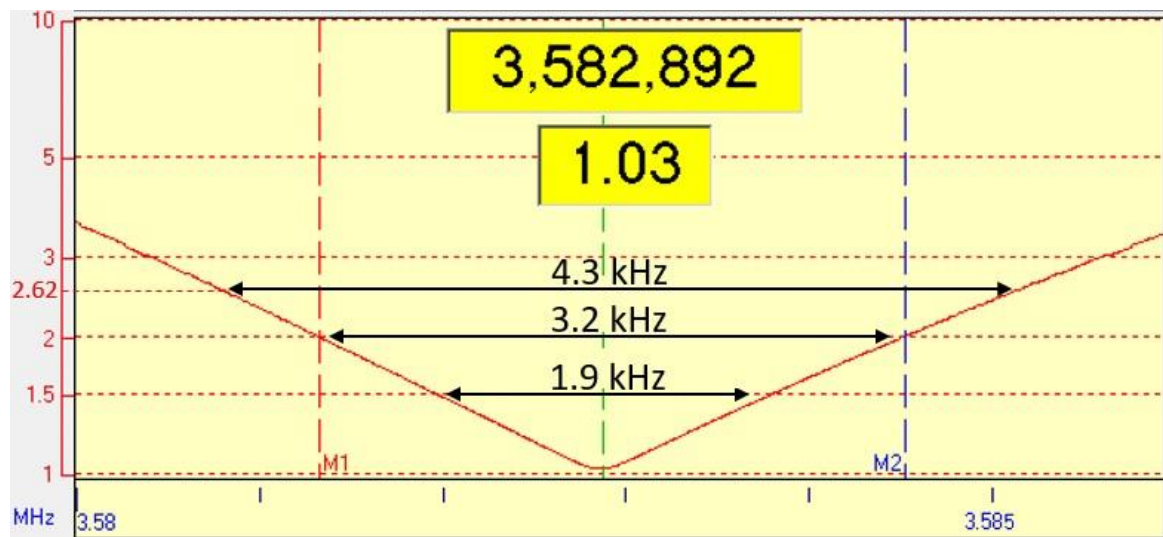
Fig. 86A: SWR vs. frequency in the 80m band
