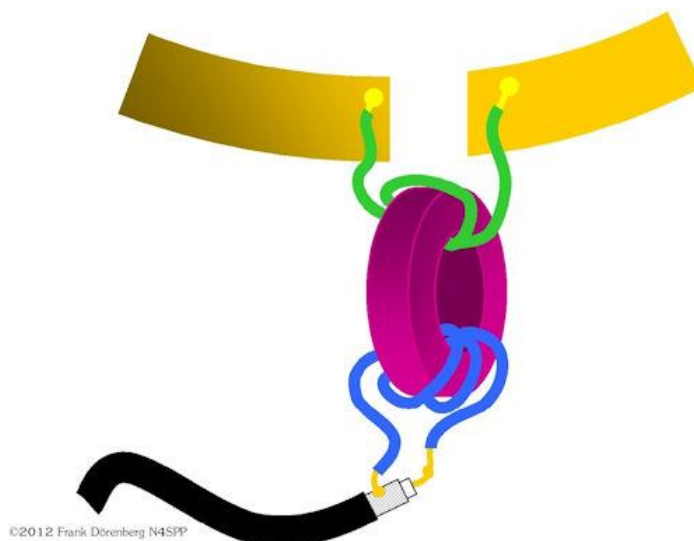
Fig. 31: N:M transformer coupling with a ferrite core
