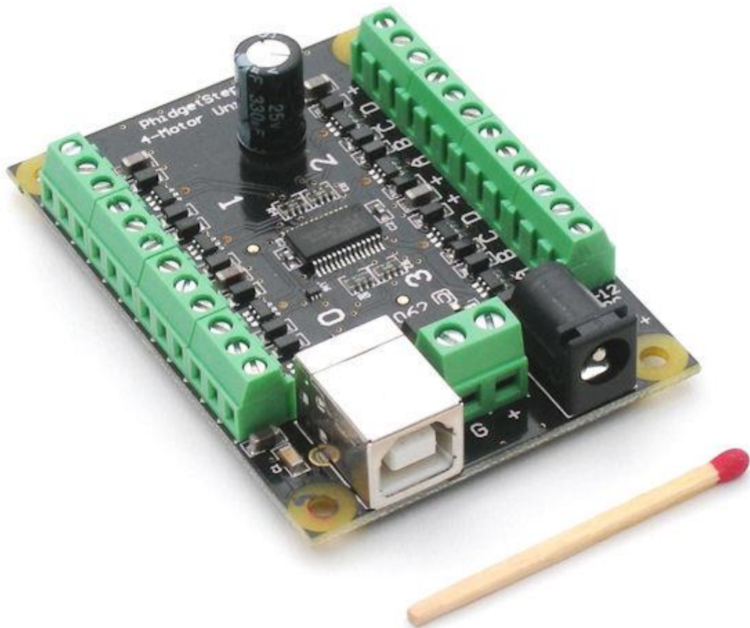
Fig. 94: The small USB controller board for four uni-polar stepper-motors
