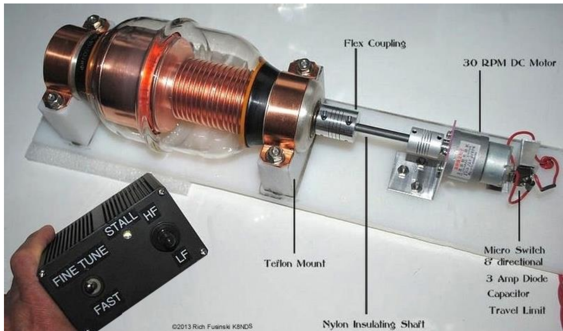
Fig. 110: Motor-drive with end-stop protection by Rich Fusinski (K8NDS) (source: ref. 11A)
