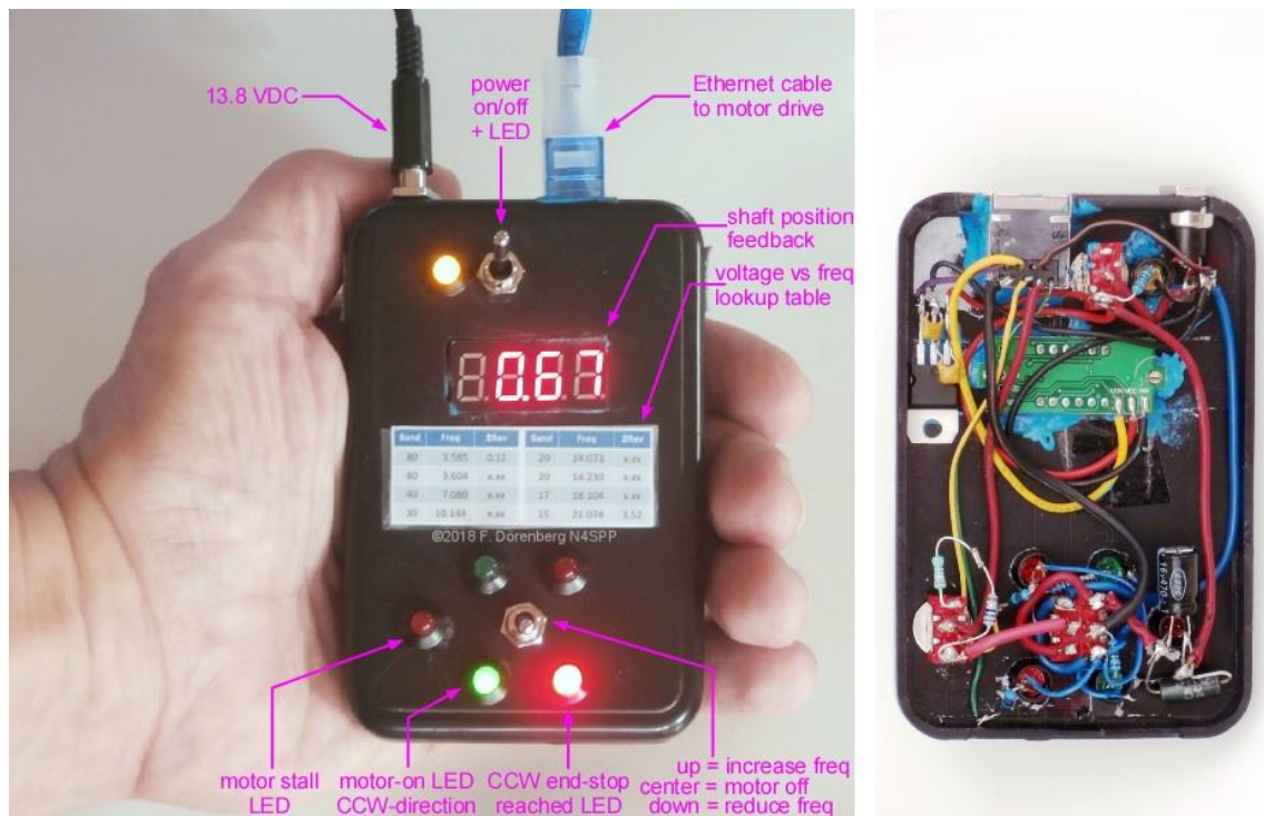
Fig. 125: The prototype remote control box, and the "ugly style" wiring (the project box measures 7x10.5x2 cm; high-low speed switch and the associated resistor is not shown in the left-hand photo)
