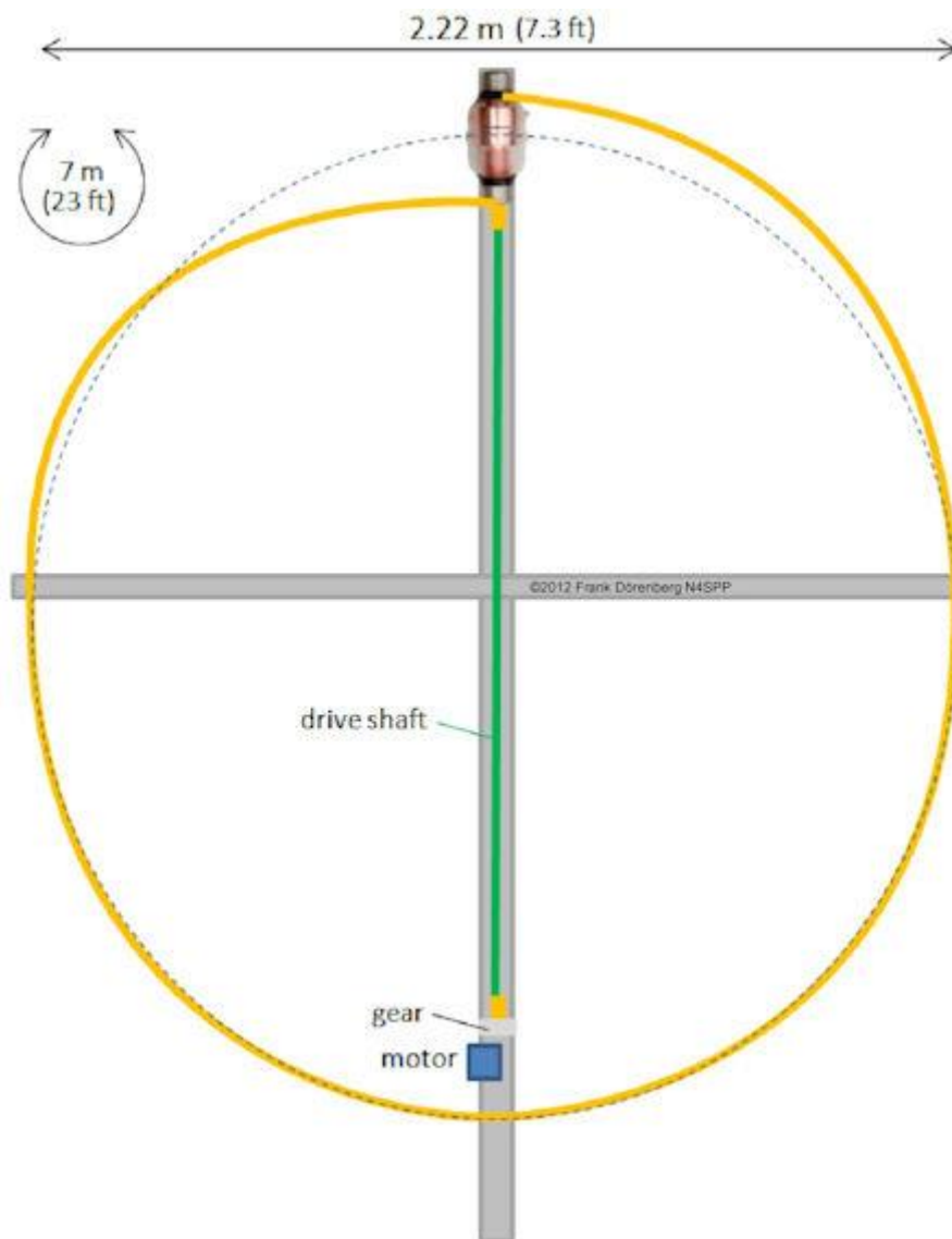
Fig. 74: Diagram of my second STL
