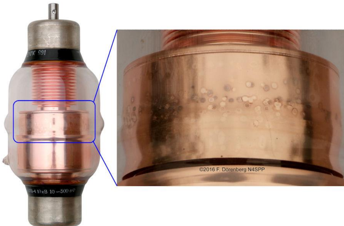
Fig. 16: A vacuum capacitor with typical over-voltage arcing damage (the round damage spots are about 4 mm ( \approx 1/6 inch) in diameter)
