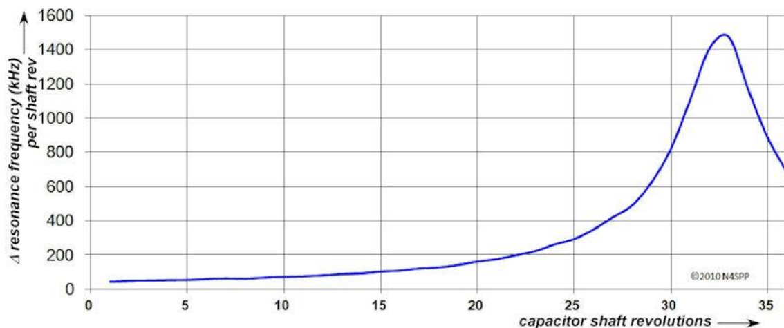
Fig. 67: Non-linear change in resonance frequency vs. varco shaft position (coupling with FT-140-43 ferrite core)
