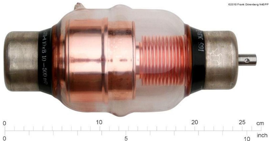
Fig. 14: My vacuum capacitor
