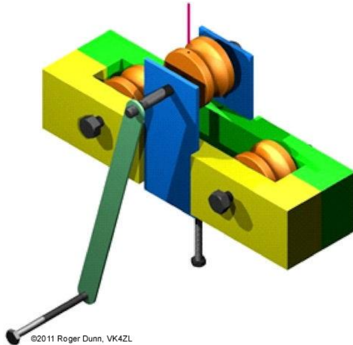
Fig. 74: A tube bender built by Roger Dunn (VK4ZL) (description: ref. 10; photos and image used with permission)
