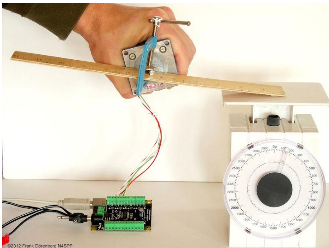
Fig. 92: Determining the break-away torque value of my SS25 motor
