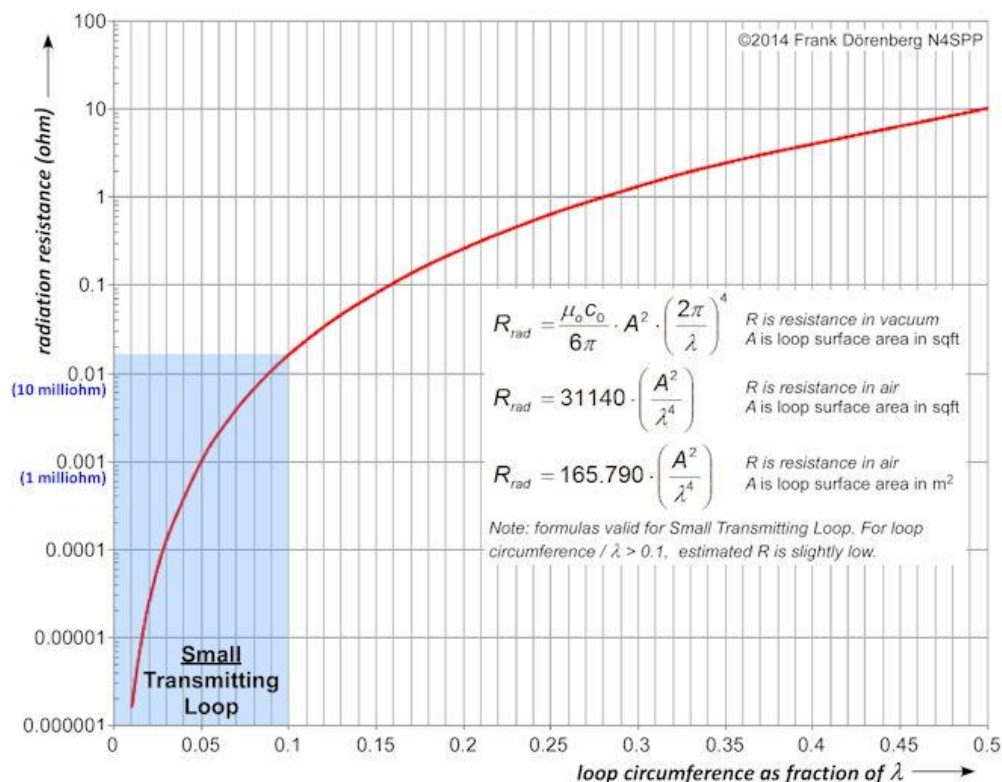
Fig. 2: Radiation resistance of a Small Transmitting Loop antenna
