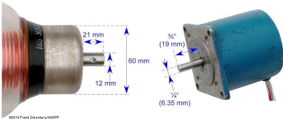
Fig. 95: Shaft dimensions of my capacitor and motor
