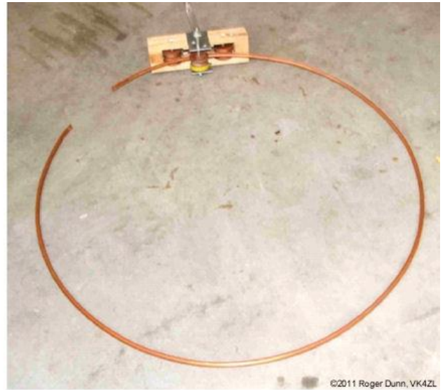
Fig. 74: A tube bender built by Roger Dunn (VK4ZL) (description: ref. 10; photos and image used with permission)
