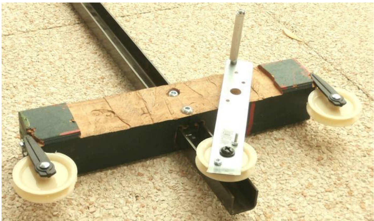
Fig. 77: An adjustable tube bender that I made for my third (smaller) STL (my third STL is made of 12 mm (0.5") soft copper tubing)
