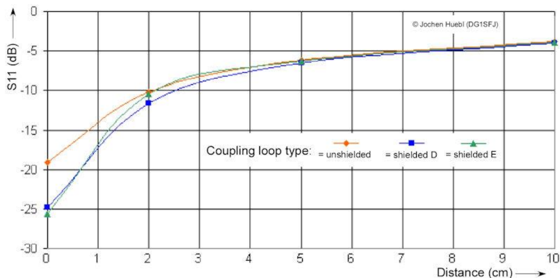
Fig. 23: Return-loss S_{11} as a function of distance between coupling loop and main loop
