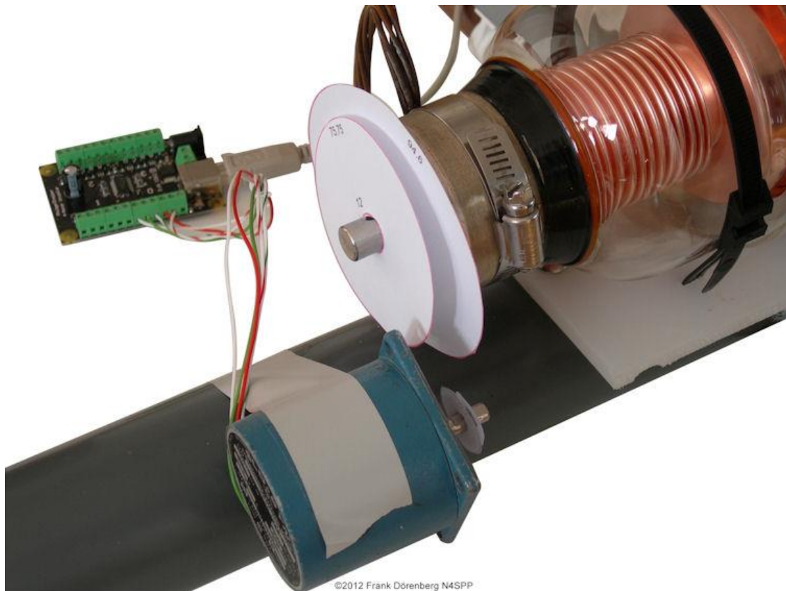
Fig. 99: paper disk "pulley" on the motor and capacitor shaft to check dimensions and clearances
