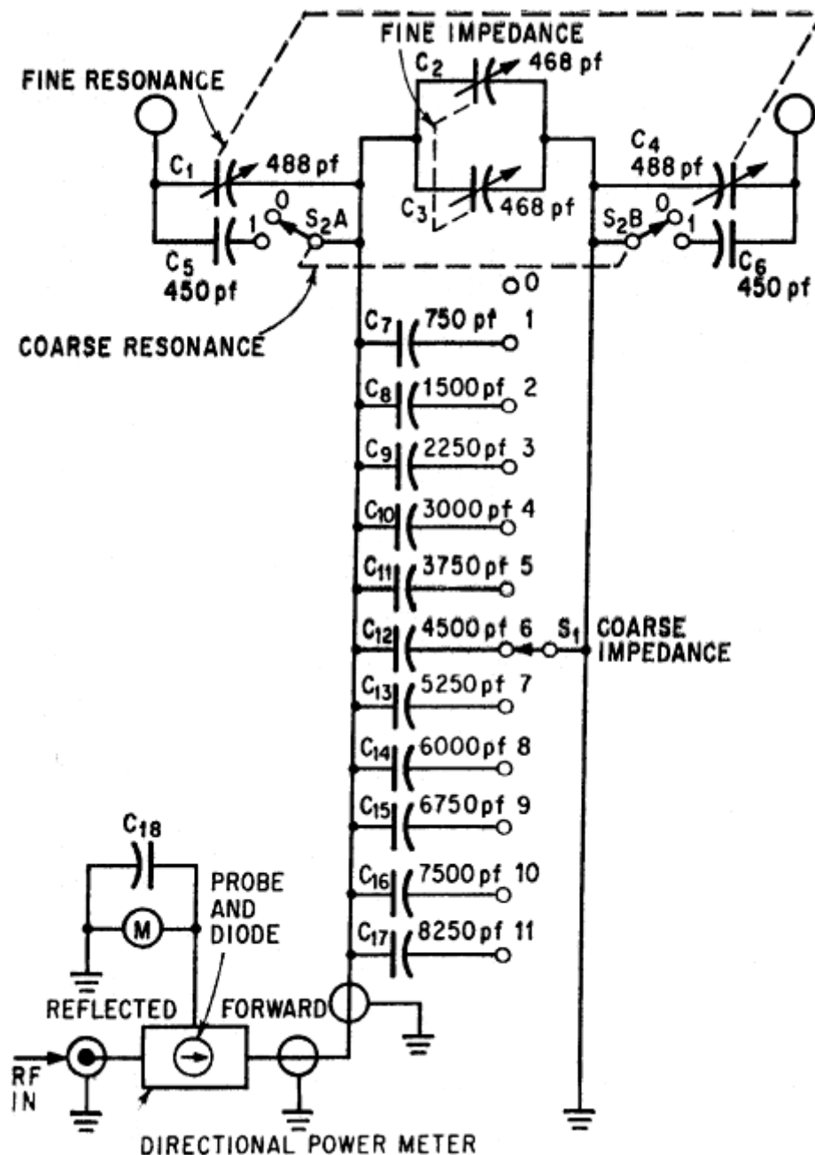
Fig. 25B: The tuning & matching unit of the "Patterson" Loop (note that tuning is done based on maximizing the antenna current, not minimizing SWR)
