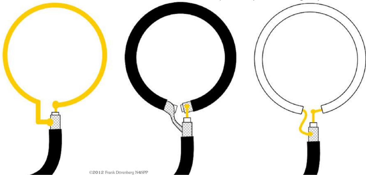
Fig. 17: Un-shielded coupling loops (solid wire, braid of coax, center-conductor of coax)
