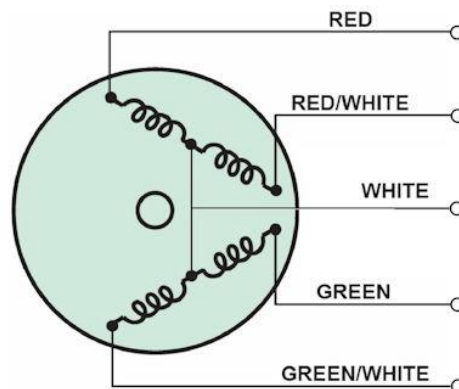
Fig. 93: Wiring of the SS25
