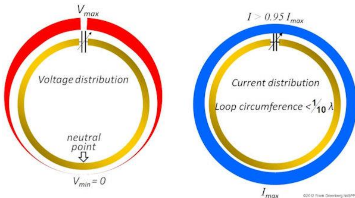
Fig. 32: Voltage and current distribution of an STL antenna
