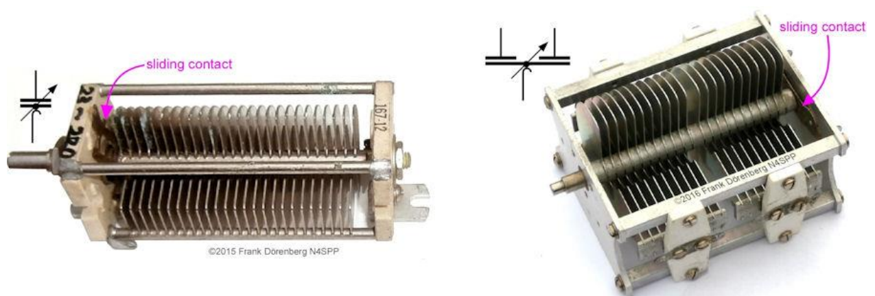
Fig. 11A: Single-section and dual-section capacitor
