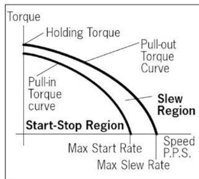
Fig. 91: Typical shape of the torque curves
