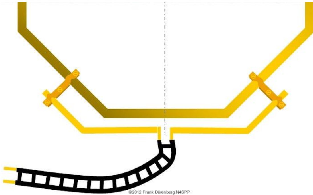
Fig.38: T-match coupling
