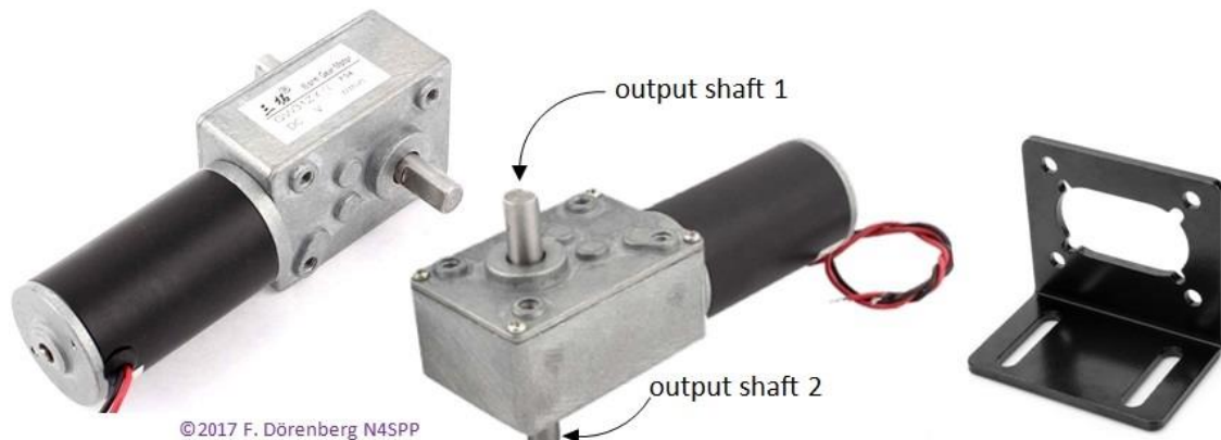
Fig. 112: The 35 rpm / 12 VDC motor and a matching mounting bracket
