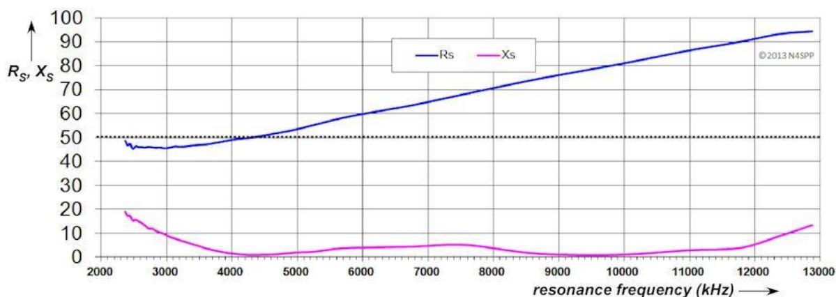
Fig. 81: Coupling transformer: FT240-31 ferrite core with 2 secondary turns, 1:1 current choke at feedpoint
