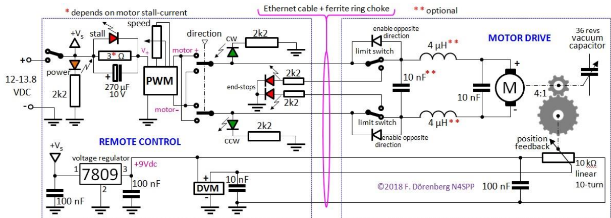
Fig. 127: Remote control schematic - with PWM variable speed adjustment
