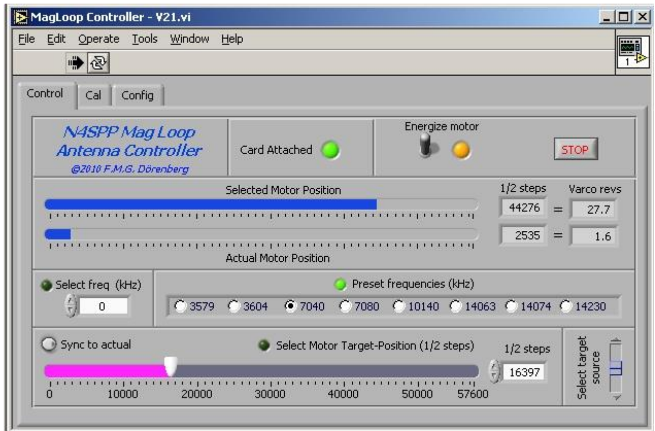
Fig. 107: The "Control" tab of the GUI of my varco motor-drive control software
