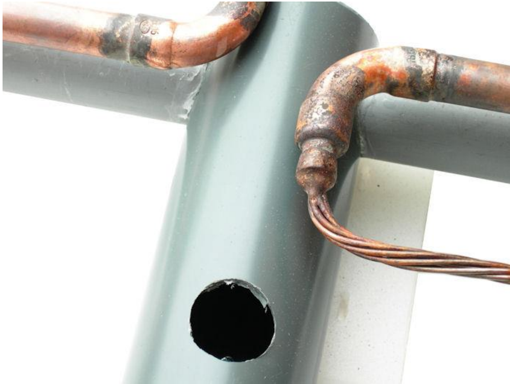
Fig. 49: Close-up of the capacitor connection wire, brazed to a copper reduction piece on the loop-ends
