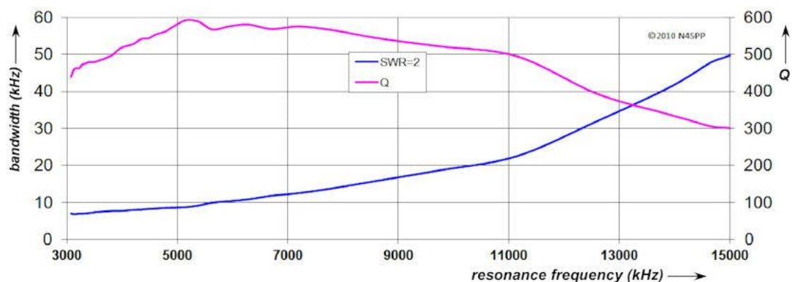
Fig. 68: Bandwidth & Q - transformer coupling with FT-140-43 core and 14 secondary turns
