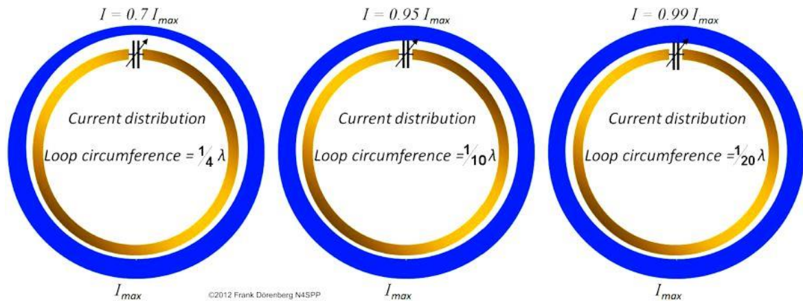
Fig. 4: Current distribution around a loop antenna (note: a circumference > 0.1 \lambda is not "small")
