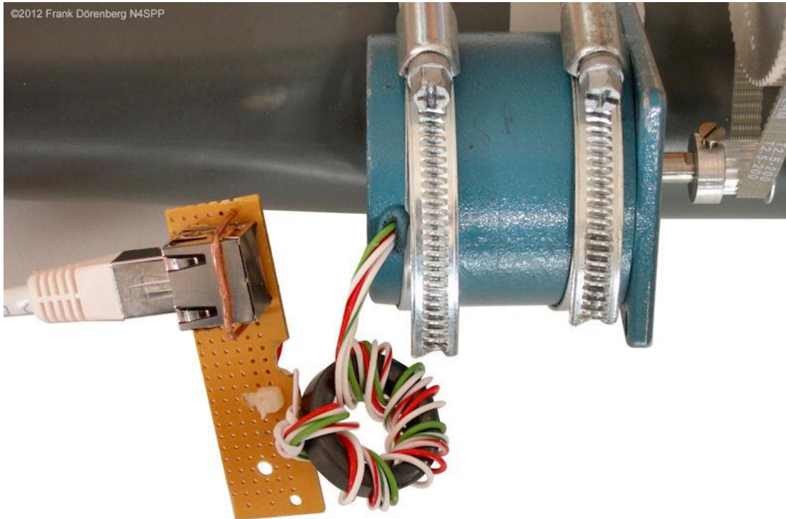
Fig. 104: A second ferrite ring current choke is placed at the motor
