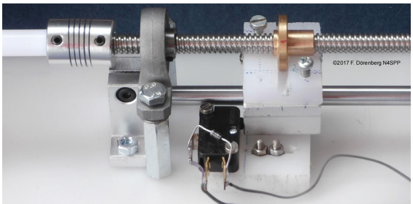
Fig. 119: Close-up view of one end-stop with micro-switch, actuated by the sliding block
