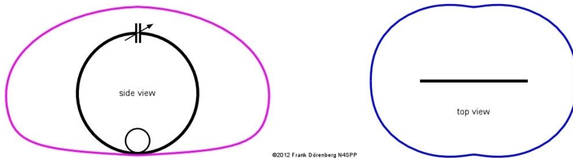
Fig. 5: approximate radiation pattern of a vertically oriented Small Transmitting Loop (circumference = 0.15 \lambda , installed 0.08 \lambda above ground)
