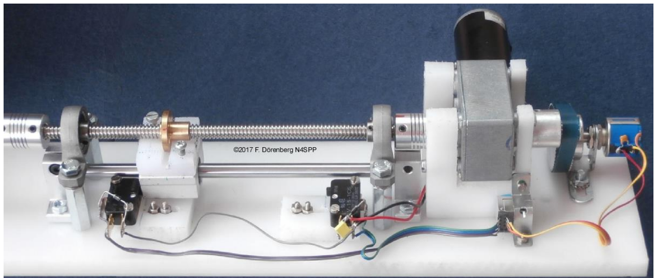
Fig. 118: Close-up view of the drive shaft, end-stop slide, motor, and position feedback potmeter
