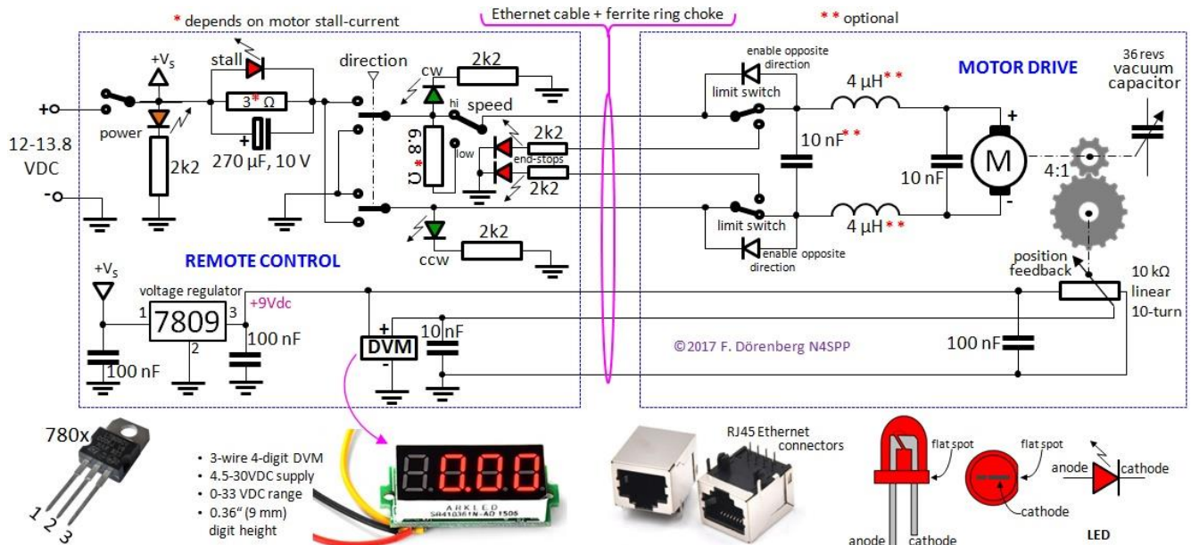
Fig. 124: Remote control schematic - with simple high/low speed selection
