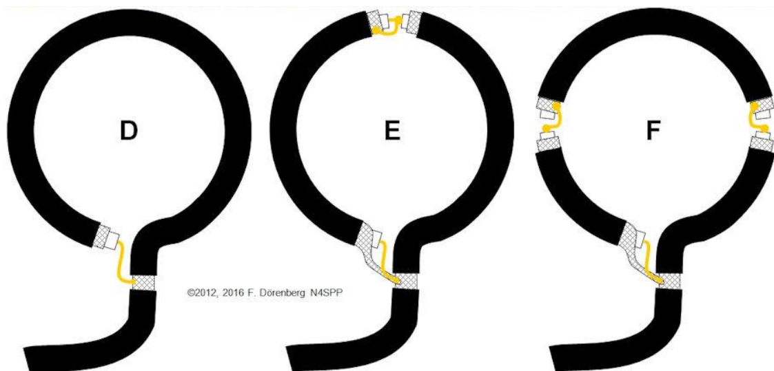
Fig. 21B: Variations of shielded coupling loops (continued)
