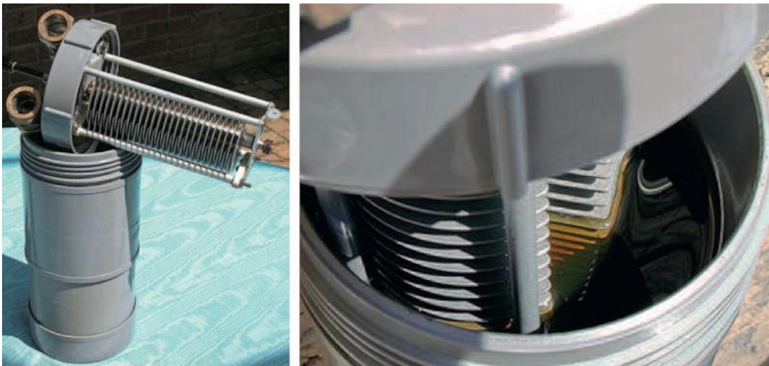
Fig. 12: Air-variable capacitor immersed in oil - doubles capacitance and voltage rating (source: ref. 12A)
