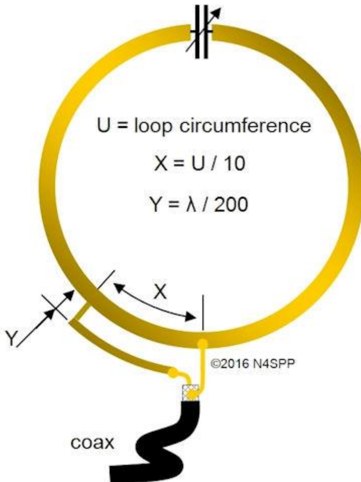
Fig. 35: Nominal dimensions for the Gamma Rod coupling (source: adapted from ref. 6N)
