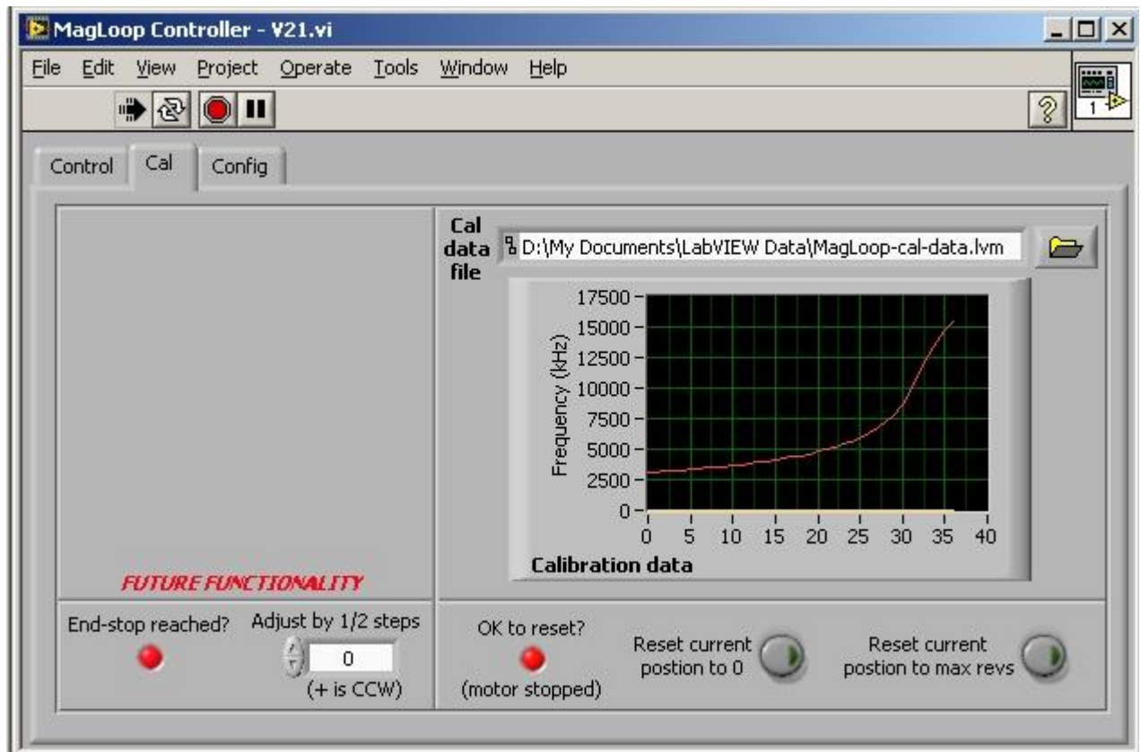
Fig. 109: The "Cal" tab of the GUI of my varco motor-drive control software
