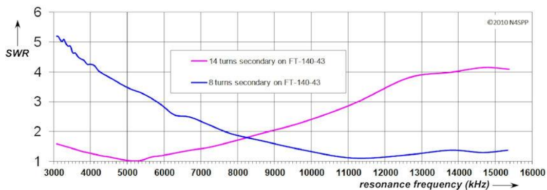
Fig. 28: SWR plot of my first STL antenna (80-20) , with a ferrite transformer core FT-140-43
