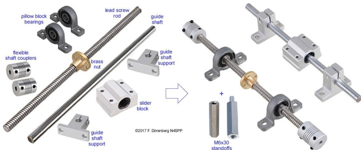
Fig. 113: The assembly for converting shaft rotation to linear motion - for actuating the end-stop switches
