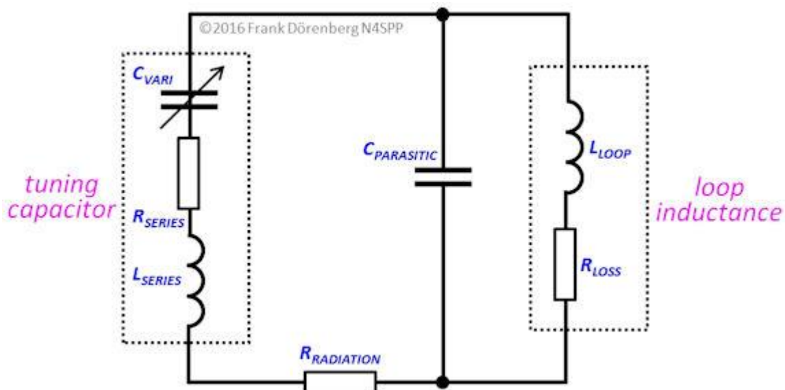
Fig. 1: Simplified equivalent lumped-element electrical circuit of an STL
