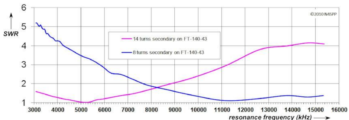
Fig. 65: Coupling transformer: FT-140-43 ferrite core with 8 & 14 secondary turns (bottom of the antenna loop is placed 80 cm (2.5 ft) above ground)
