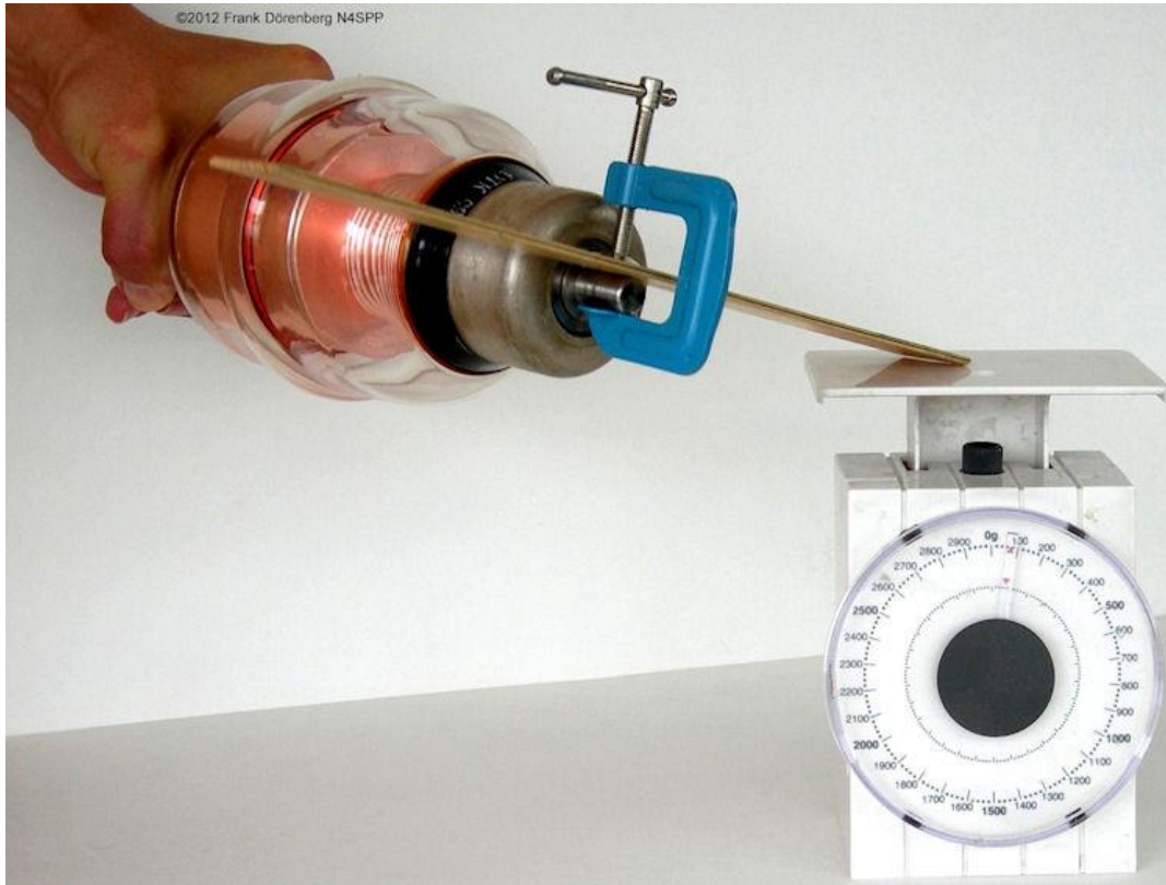
Fig. 88: Determining the torque values of my capacitor
