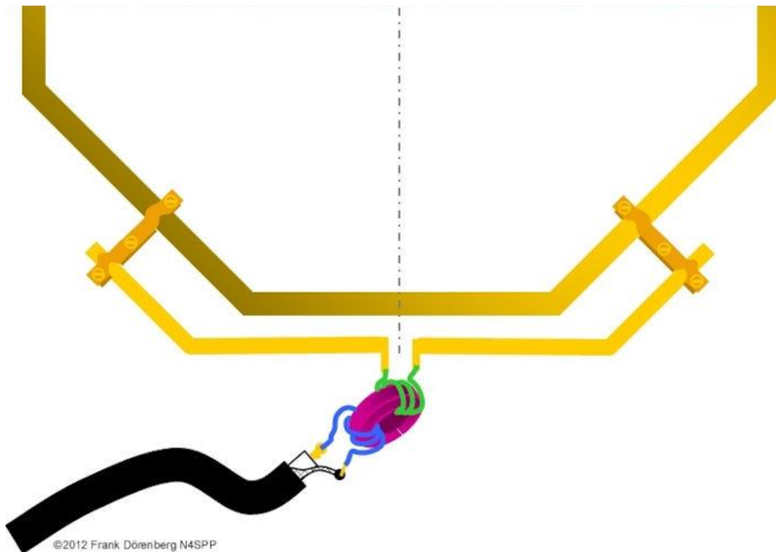
Fig. 39: T-Match coupling combined with N:M transformer
