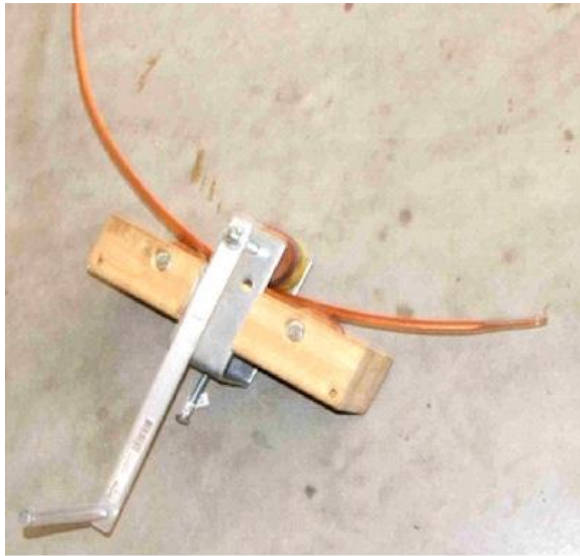
Fig. 74: A tube bender built by Roger Dunn (VK4ZL) (description: ref. 10; photos and image used with permission)
