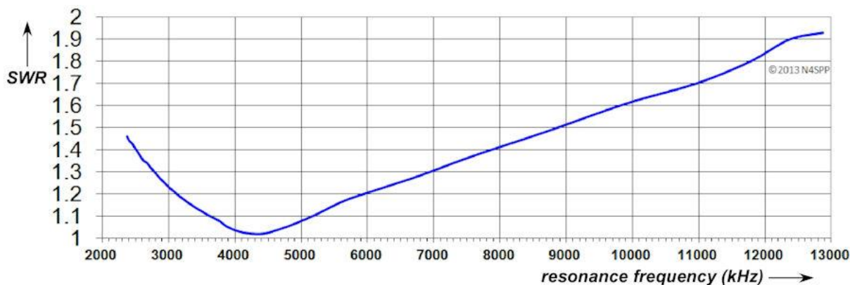
Fig. 80: Coupling transformer: FT240-31 ferrite core with 2 secondary turns, 1:1 current choke at feedpoint
