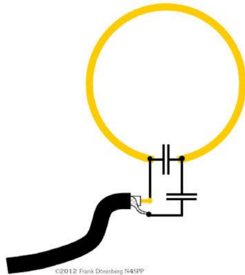
Fig. 18: Un-shielded coupling loop with a tuning and a loading capacitor
