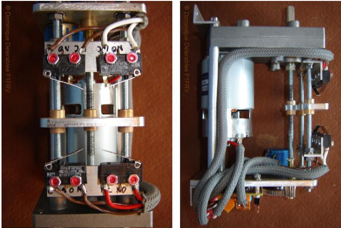
Fig. 111: Top view & side view of a motor-drive by Dominique Delerabee (F1FRV) (source: ref. 12F)
