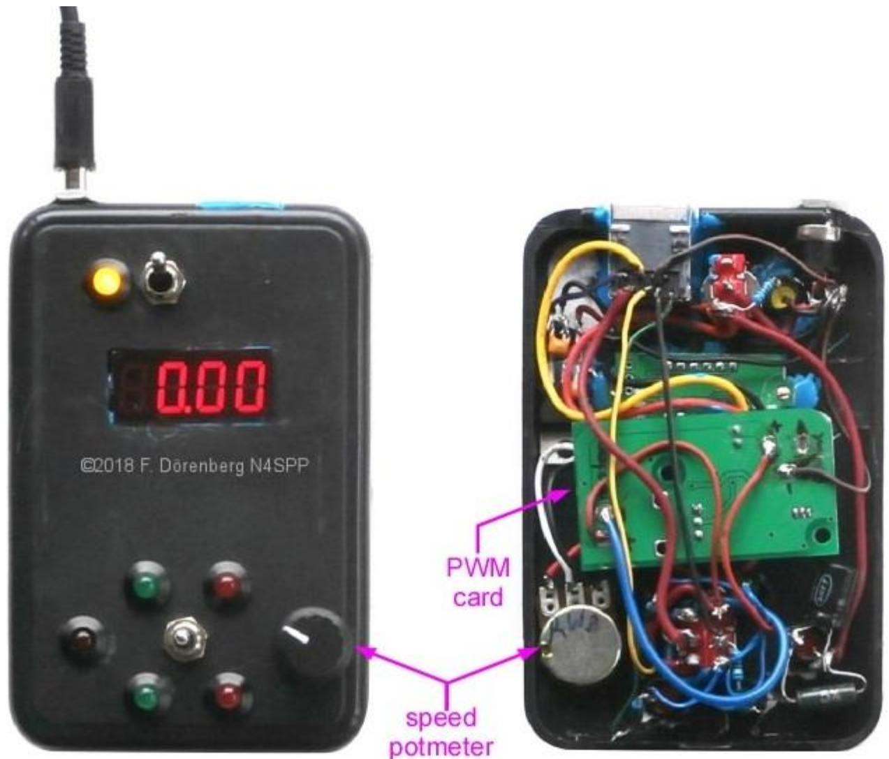
Fig. 128: The prototype remote control box - now with variable speed adjustment (red contrast filter added to the 4-digit DVM display)
