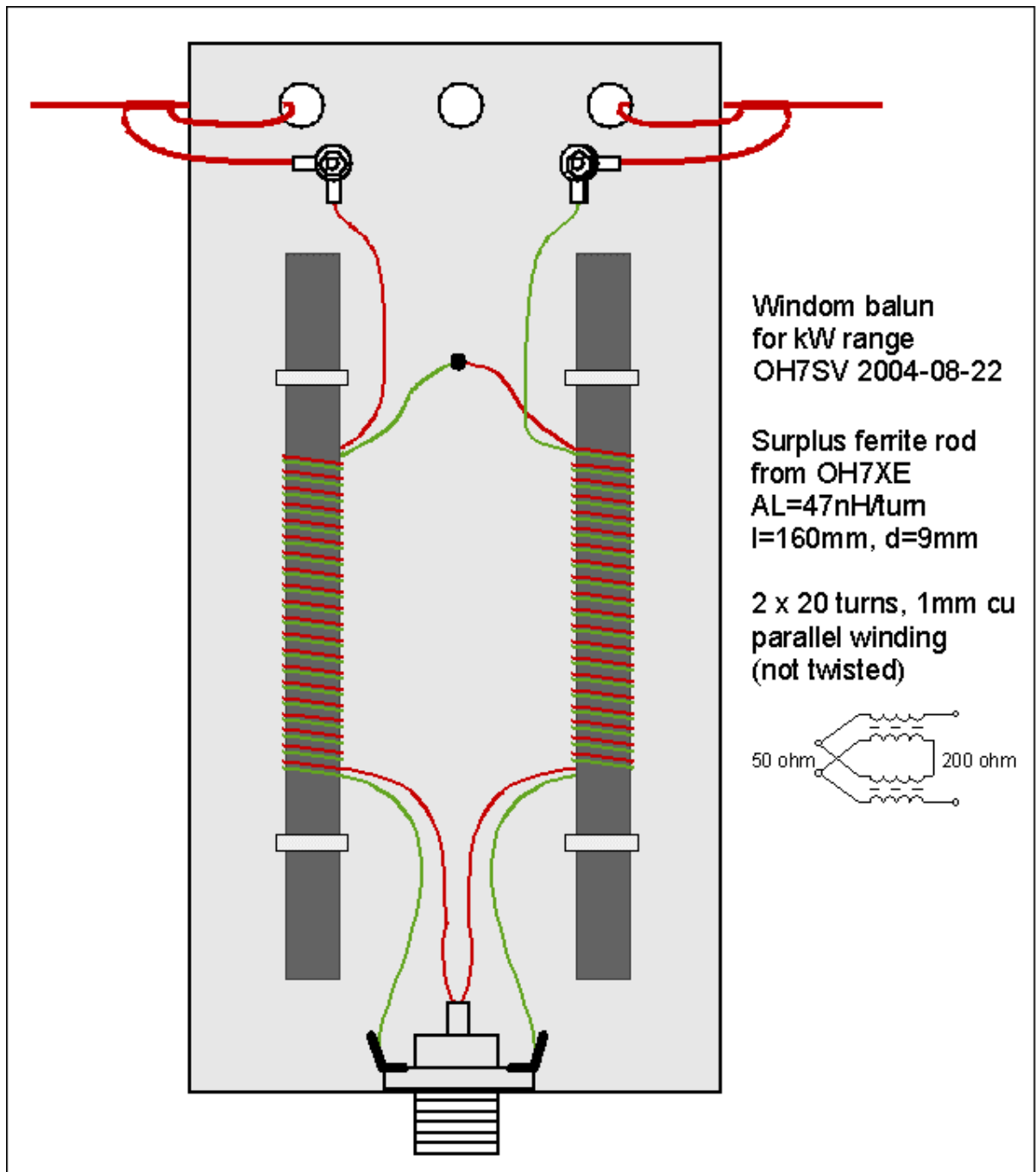
Window balun made with surplus ferrite rods
