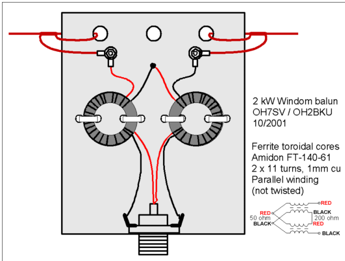
Windom balun made with Amidon ferrite toroids
