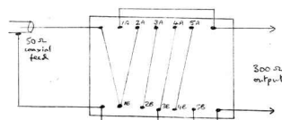
5:2 wideband transformer wiring diagram
