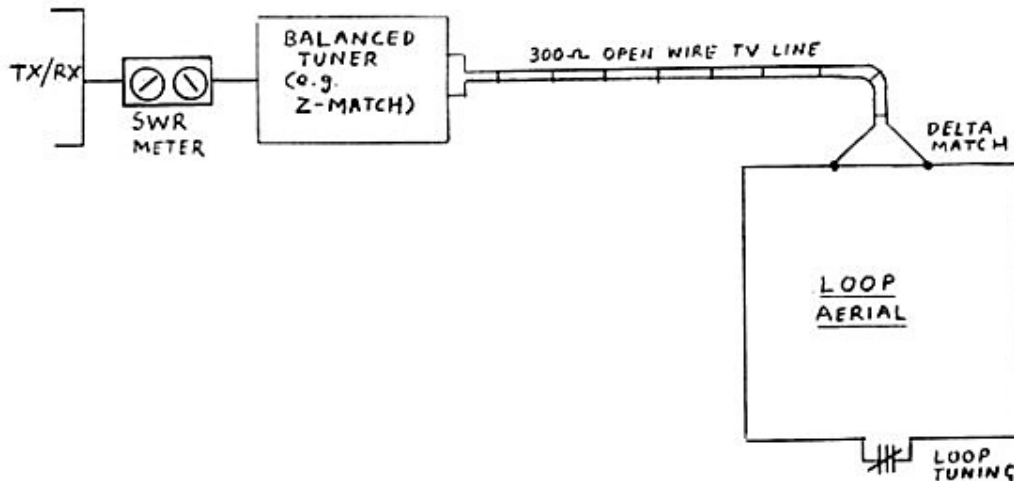
Figure 3 Matching System using Open Wire TV Line
