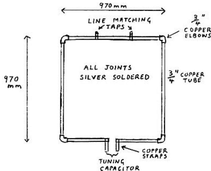
Figure 2 Loop Assembly
